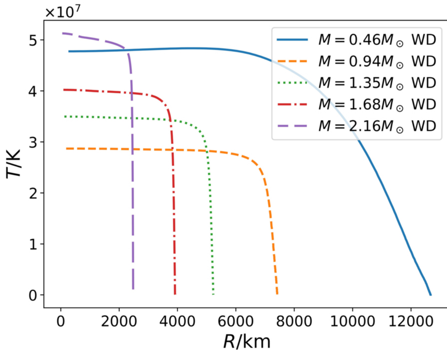
Figure C1. from Zenia Zuraig et al 2026 Astrophys. J. Lett. 1010 doi:10.3847/2041-8213/aea97e https://dx.doi.org/10.3847/2041-8213/aea97e © 2026. The Author(s). Published by the American Astronomical Society.
