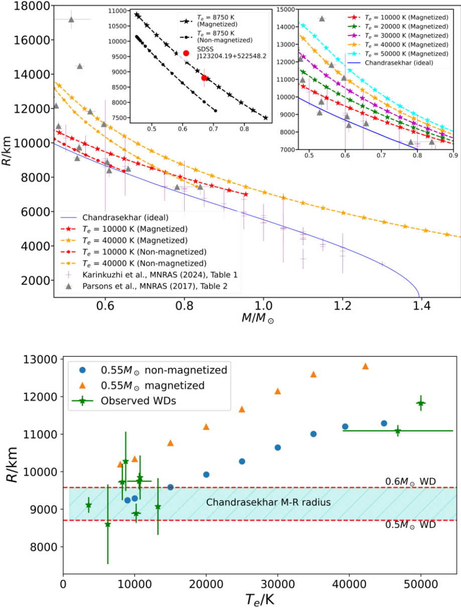
Figure 4. from Zenía Zuraíq et al 2026 Astrophys. J. Lett. 1010 doi:10.3847/2041-8213/aea97e https://dx.doi.org/10.3847/2041-8213/aea97e © 2026. The Author(s). Published by the American Astronomical Society.
