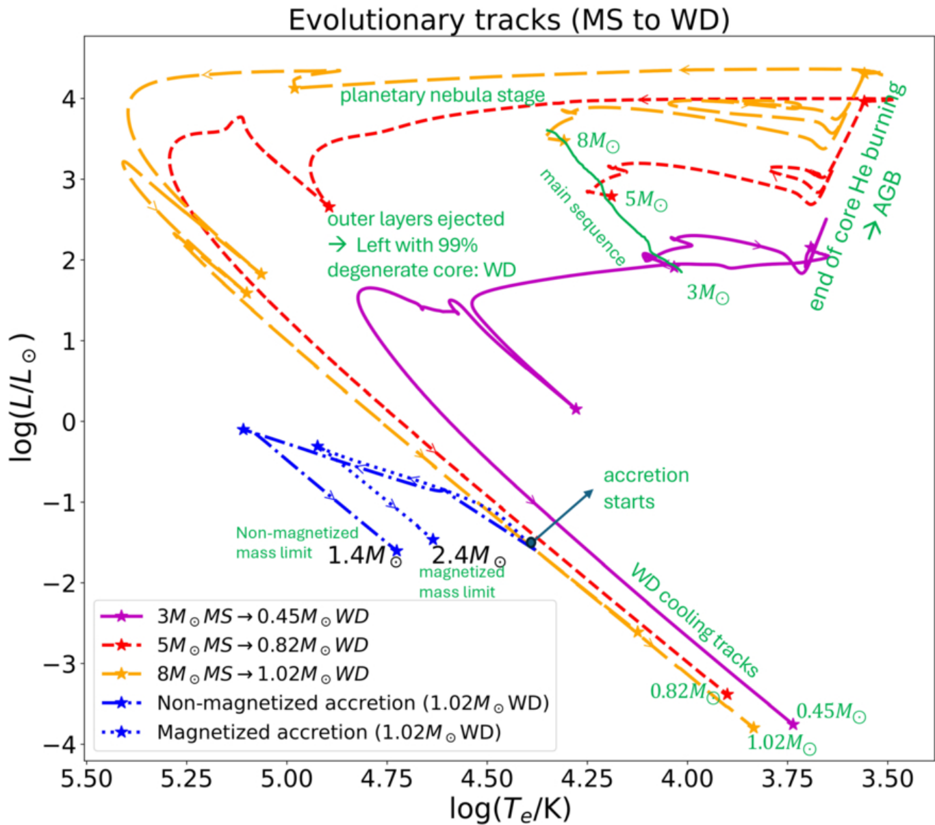
Figure 1. from Zenía Zuraig et al 2026 Astrophys. J. Lett. 1010 doi:10.3847/2041-8213/aea97e https://dx.doi.org/10.3847/2041-8213/aea97e © 2026. The Author(s). Published by the American Astronomical Society.
