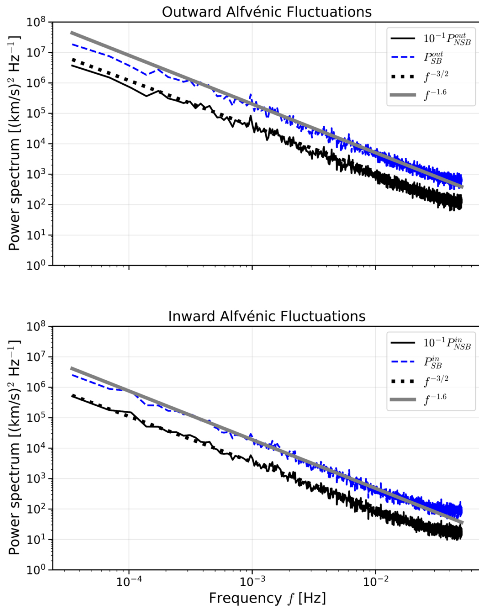
Figure 4. from Sofiane Bourouaine 2026 Astrophys. J. Lett. 1010 doi:10.3847/2041-8213/aea90c https://dx.doi.org/10.3847/2041-8213/aea90c © 2026. The Author(s). Published by the American Astronomical Society.
