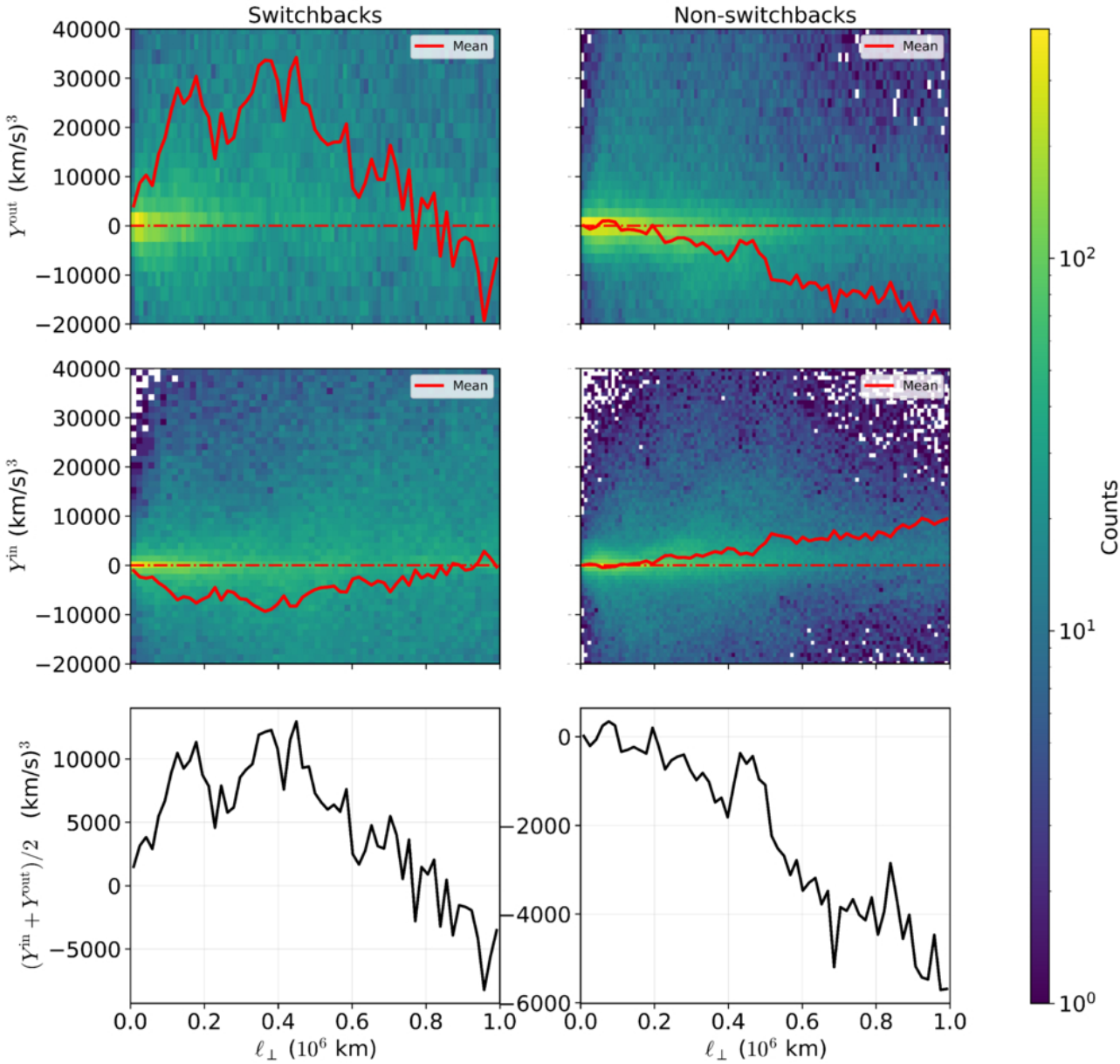
Figure 2. from Sofiane Bourouaine 2026 Astrophys. J. Lett. 1010 doi:10.3847/2041-8213/aea90c https://dx.doi.org/10.3847/2041-8213/aea90c © 2026. The Author(s). Published by the American Astronomical Society.
