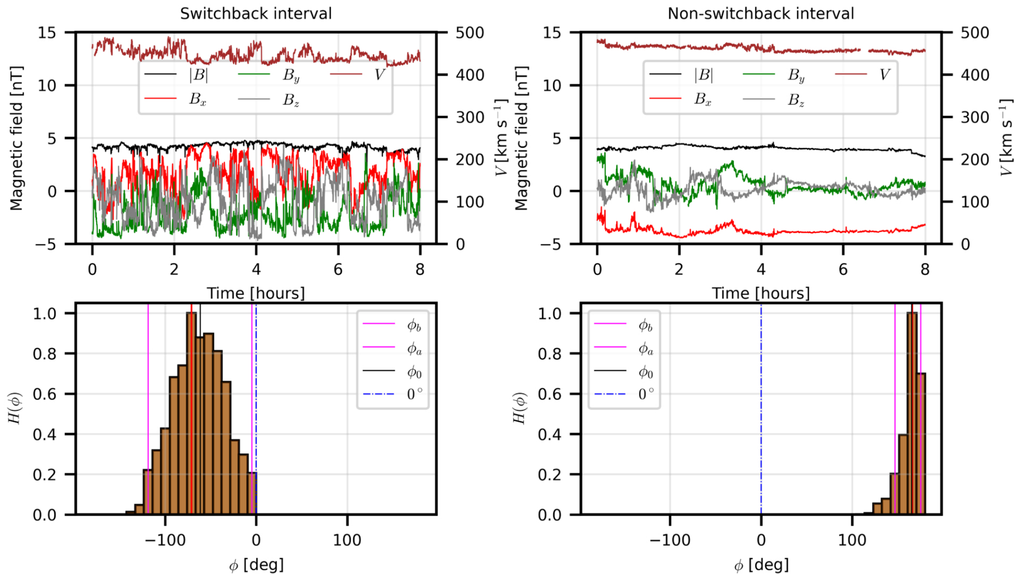
Figure 1. from Sofiane Bourouaine 2026 Astrophys. J. Lett. 1010 doi:10.3847/2041-8213/aea90c https://dx.doi.org/10.3847/2041-8213/aea90c © 2026. The Author(s). Published by the American Astronomical Society.
