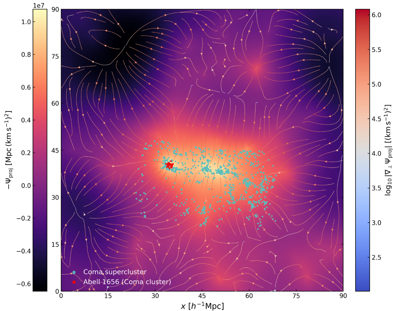
Figure 5. from Kunyao Zhao et al 2026 Astrophys. J. Lett. 1010 doi:10.3847/2041-8213/aea8fe https://dx.doi.org/10.3847/2041-8213/aea8fe © 2026. The Author(s). Published by the American Astronomical Society.
