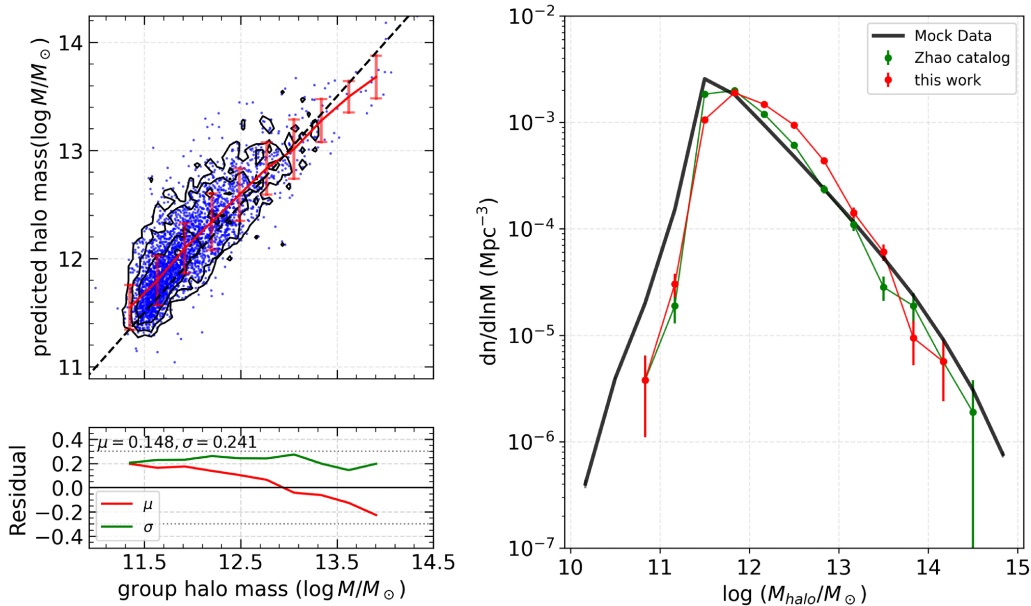
Figure 4. from Kunyao Zhao et al 2026 Astrophys. J. Lett. 1010 doi:10.3847/2041-8213/aea8fe https://dx.doi.org/10.3847/2041-8213/aea8fe © 2026. The Author(s). Published by the American Astronomical Society.
