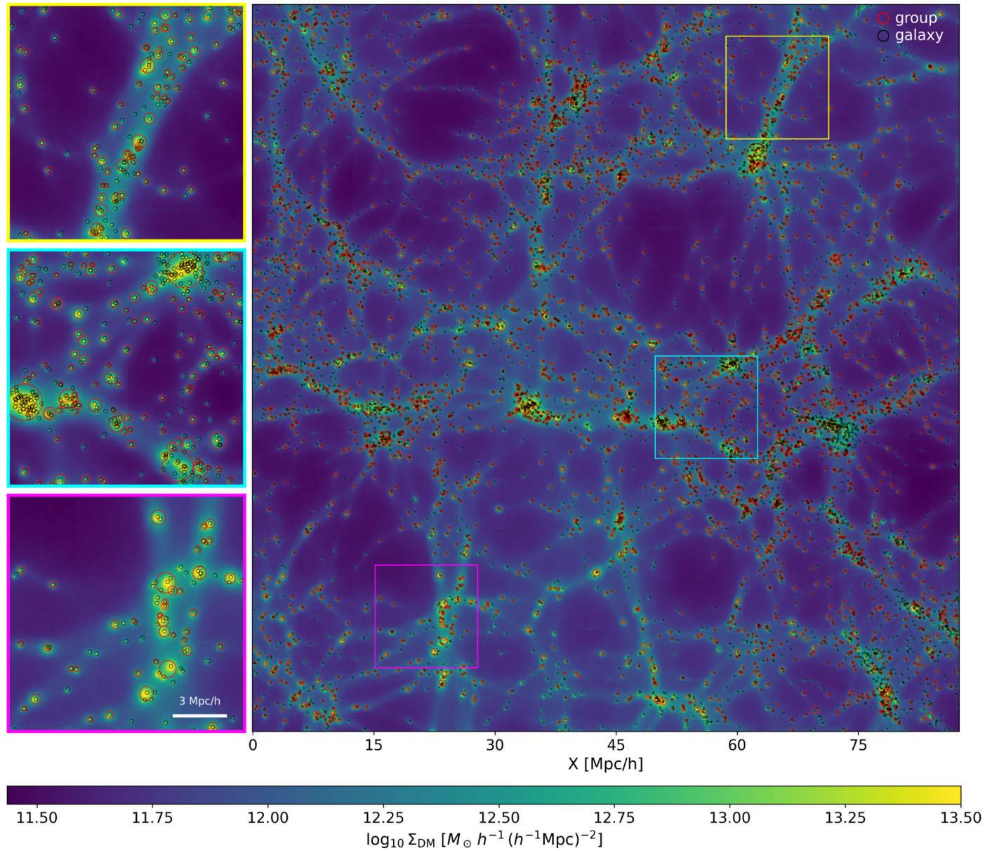
Figure 3. from Kunyao Zhao et al 2026 Astrophys. J. Lett. 1010 doi:10.3847/2041-8213/aea8fe https://dx.doi.org/10.3847/2041-8213/aea8fe © 2026. The Author(s). Published by the American Astronomical Society.
