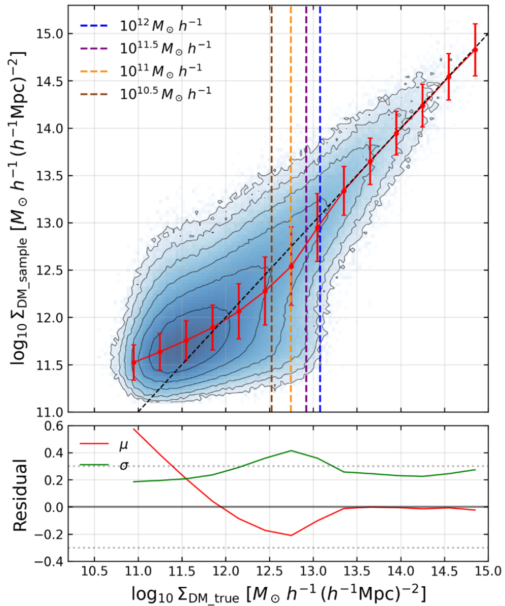
Figure 2. from Kunyao Zhao et al 2026 Astrophys. J. Lett. 1010 doi:10.3847/2041-8213/aea8fe https://dx.doi.org/10.3847/2041-8213/aea8fe © 2026. The Author(s). Published by the American Astronomical Society.
