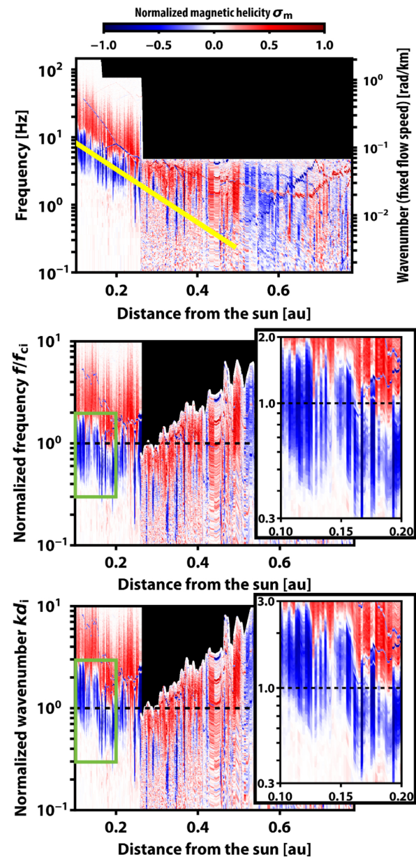
Figure 4. from Masatomi Iizawa et al 2026 Astrophys. J. Lett. 1010 doi:10.3847/2041-8213/aea84b https://dx.doi.org/10.3847/2041-8213/aea84b © 2026. The Author(s). Published by the American Astronomical Society.
