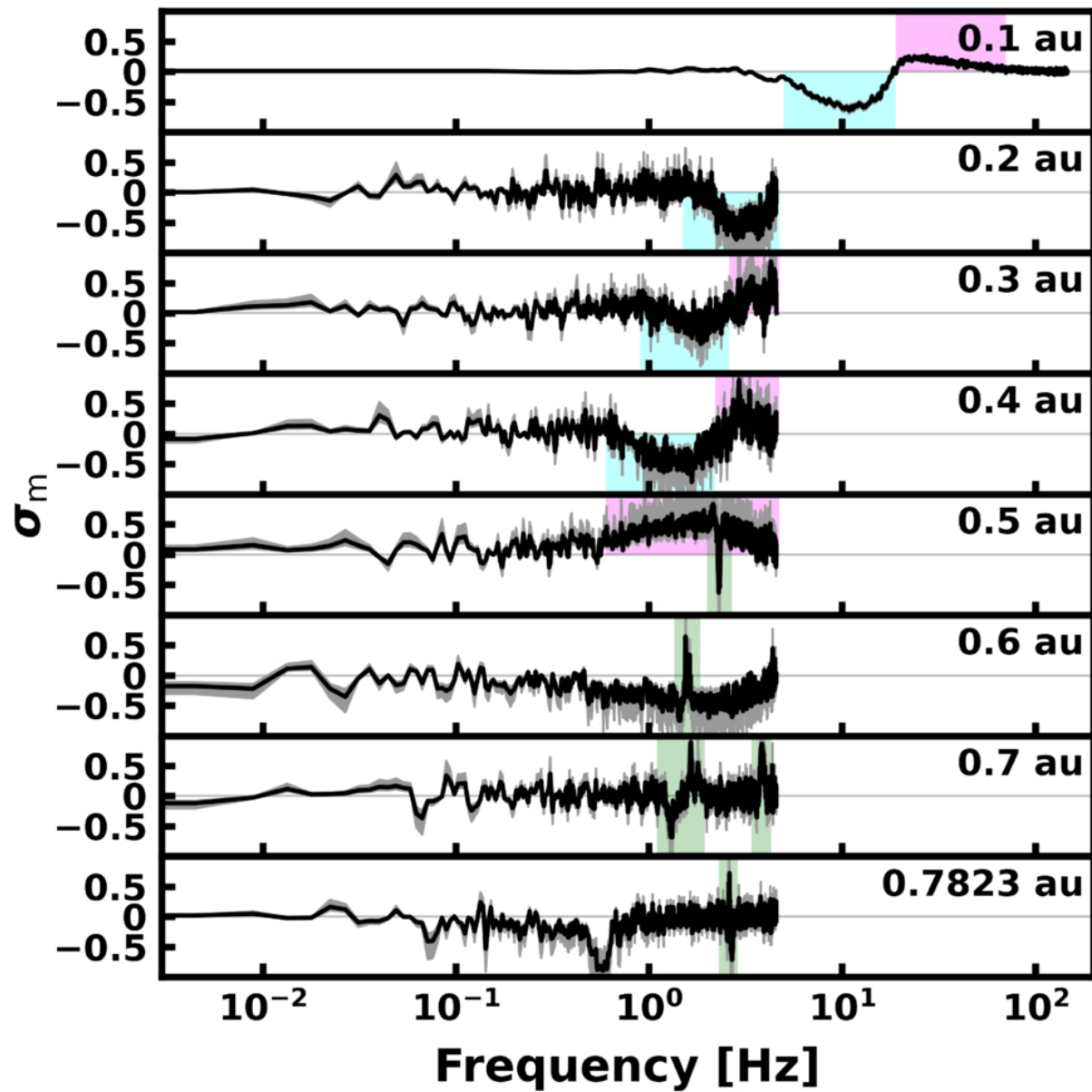
Figure 3. from Masatomi Iizawa et al 2026 Astrophys. J. Lett. 1010 doi:10.3847/2041-8213/aea84b https://dx.doi.org/10.3847/2041-8213/aea84b © 2026. The Author(s). Published by the American Astronomical Society.
