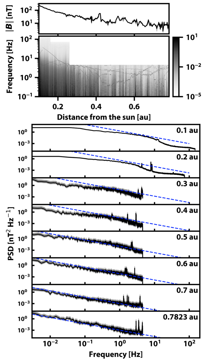
Figure 2. from Masatomi Iizawa et al 2026 Astrophys. J. Lett. 1010 doi:10.3847/2041-8213/aea84b https://dx.doi.org/10.3847/2041-8213/aea84b © 2026. The Author(s). Published by the American Astronomical Society.
