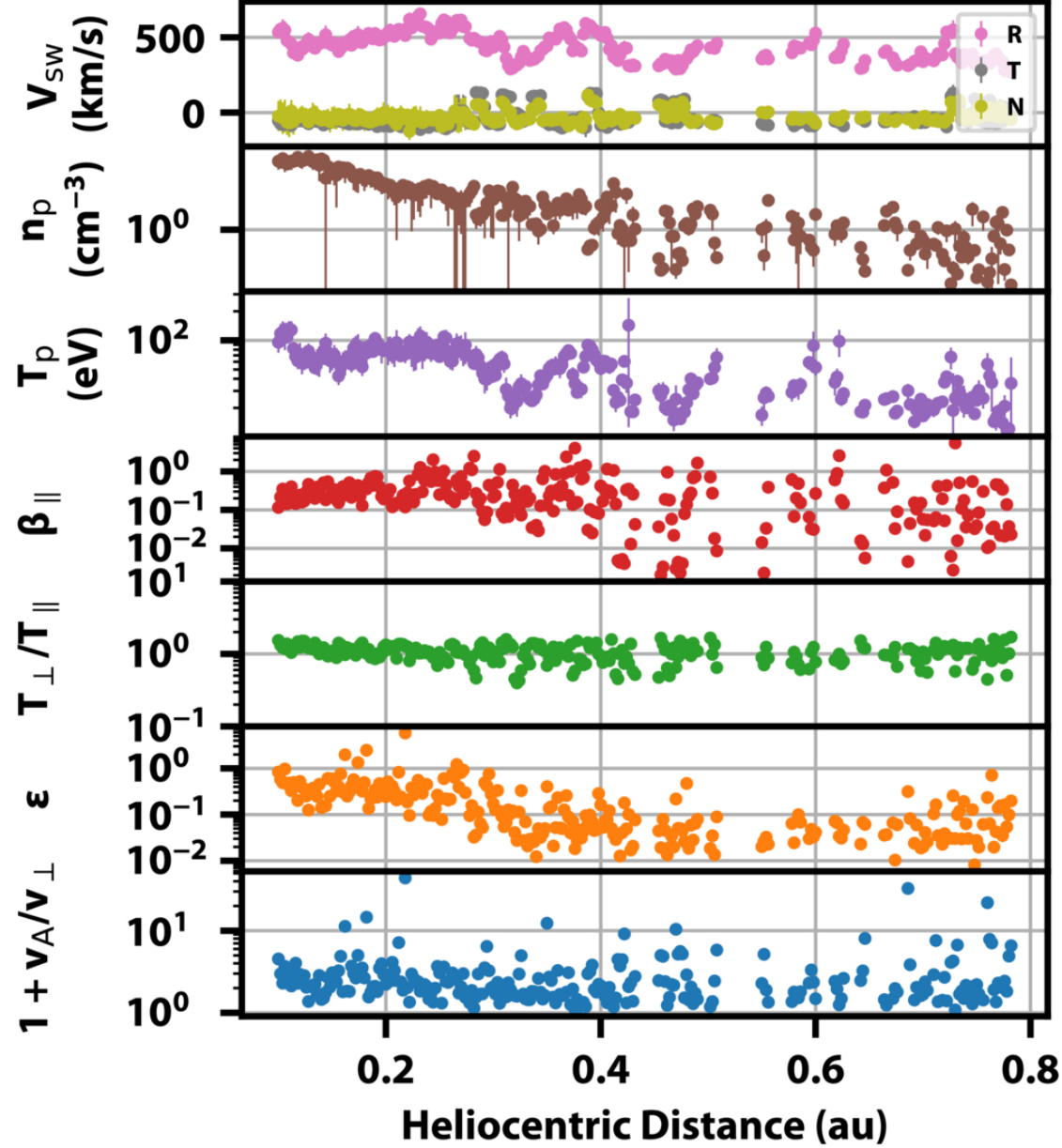
Figure 1. from Masatomi Iizawa et al 2026 Astrophys. J. Lett. 1010 doi:10.3847/2041-8213/aea84b https://dx.doi.org/10.3847/2041-8213/aea84b © 2026. The Author(s). Published by the American Astronomical Society.
