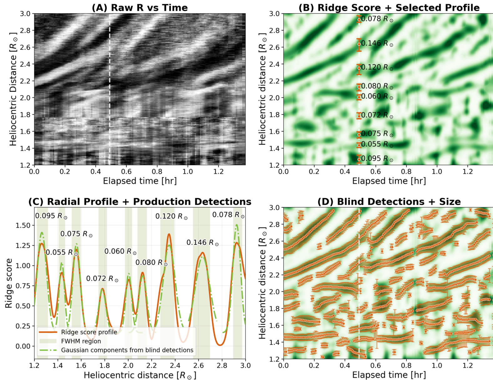
Figure 2. from Zac Bailey et al 2026 Astrophys. J. Lett. 1010 doi:10.3847/2041-8213/aea849 https://dx.doi.org/10.3847/2041-8213/aea849 © 2026. The Author(s). Published by the American Astronomical Society.
