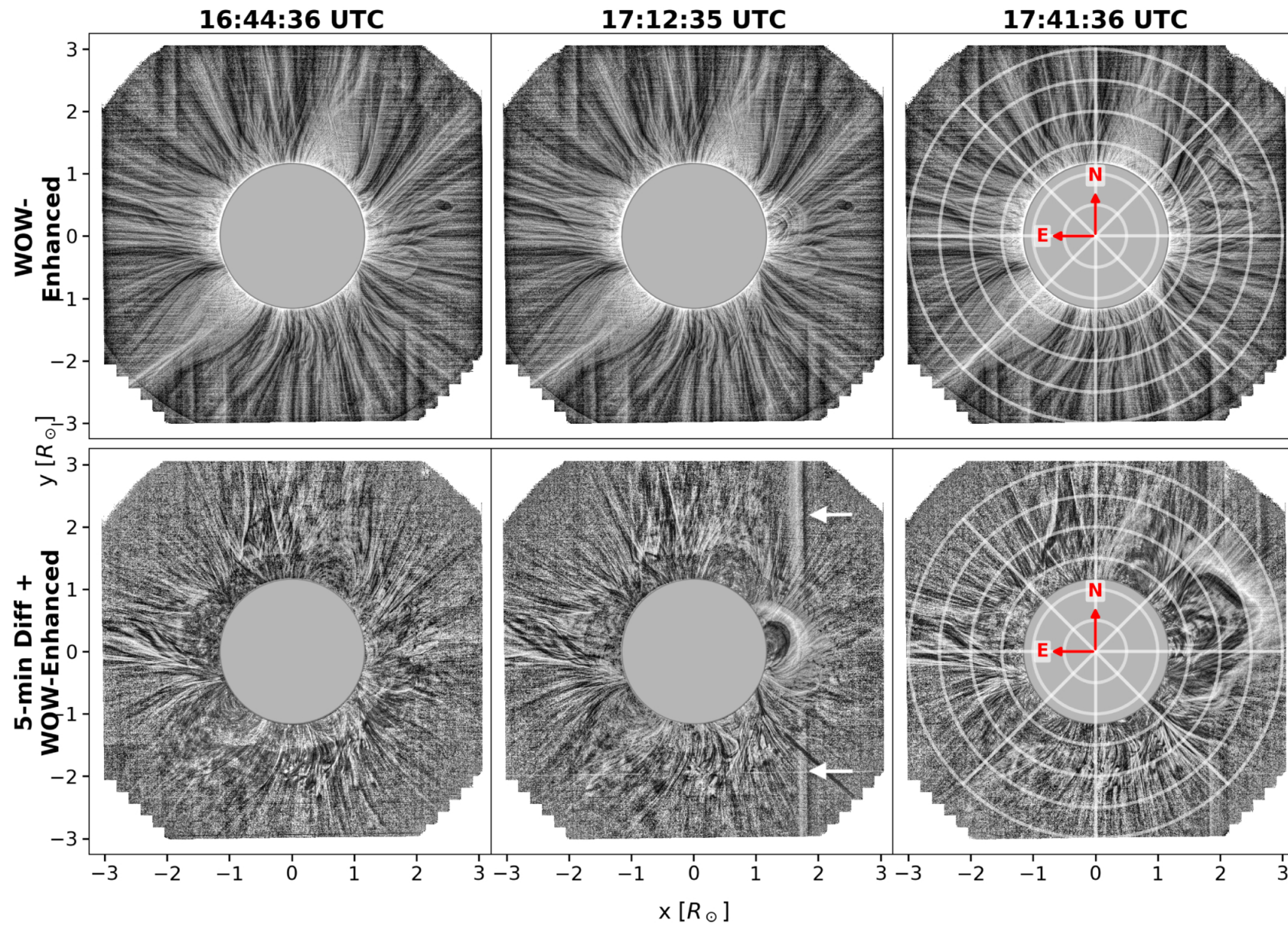
Figure 1. from Zac Bailey et al 2026 Astrophys. J. Lett. 1010 doi:10.3847/2041-8213/aea849 https://dx.doi.org/10.3847/2041-8213/aea849 © 2026. The Author(s). Published by the American Astronomical Society.
