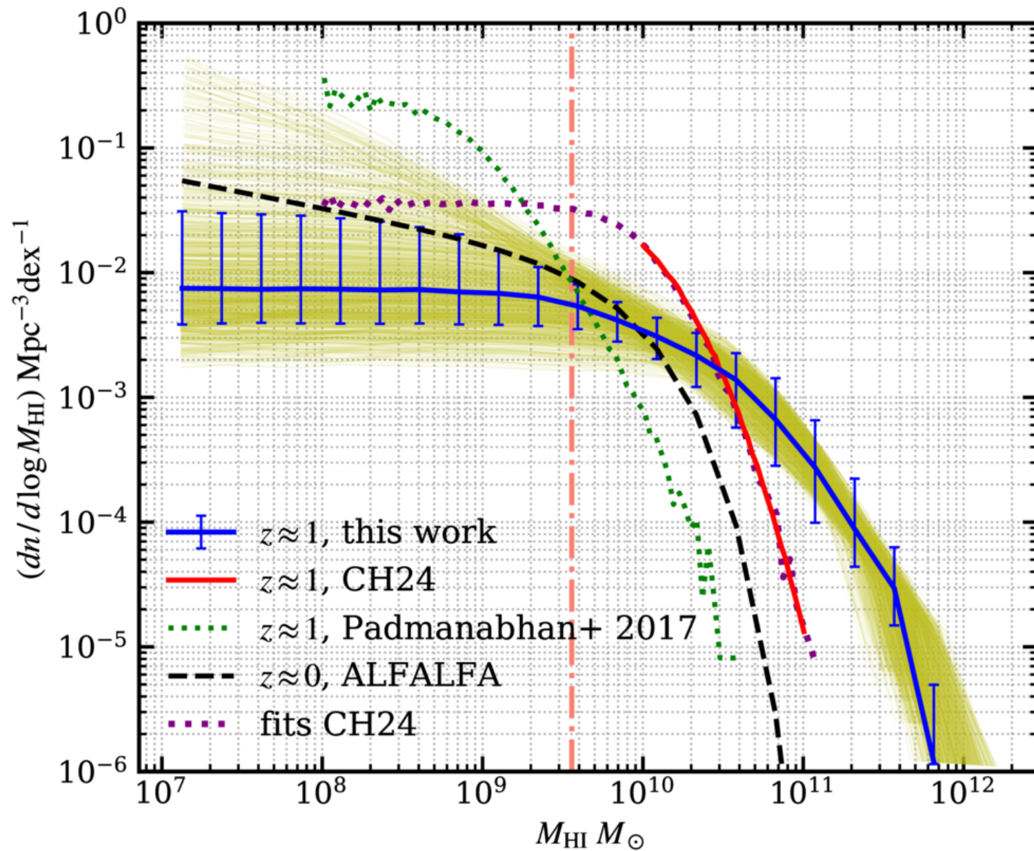
Figure 3. from Minal Chhabra et al 2026 Astrophys. J. Lett. 1009 doi:10.3847/2041-8213/aea790 https://dx.doi.org/10.3847/2041-8213/aea790 © 2026. The Author(s). Published by the American Astronomical Society.
