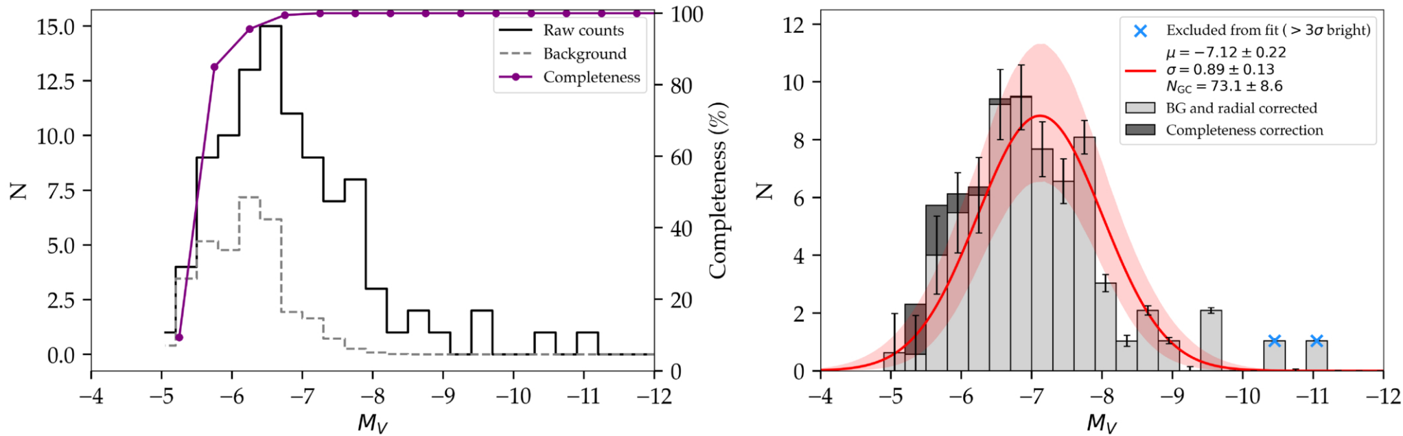
Figure 4. from Maria Luísa Buzzo et al 2026 Astrophys. J. Lett. 1009 doi:10.3847/2041-8213/aea6d2 https://dx.doi.org/10.3847/2041-8213/aea6d2 © 2026. The Author(s). Published by the American Astronomical Society.
