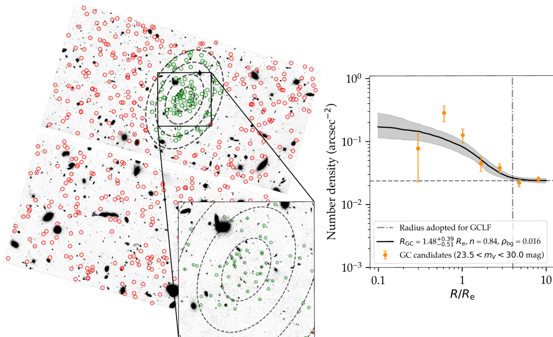
Figure 3. from Maria Luísa Buzzo et al 2026 Astrophys. J. Lett. 1009 doi:10.3847/2041-8213/aea6d2 https://dx.doi.org/10.3847/2041-8213/aea6d2 © 2026. The Author(s). Published by the American Astronomical Society.
