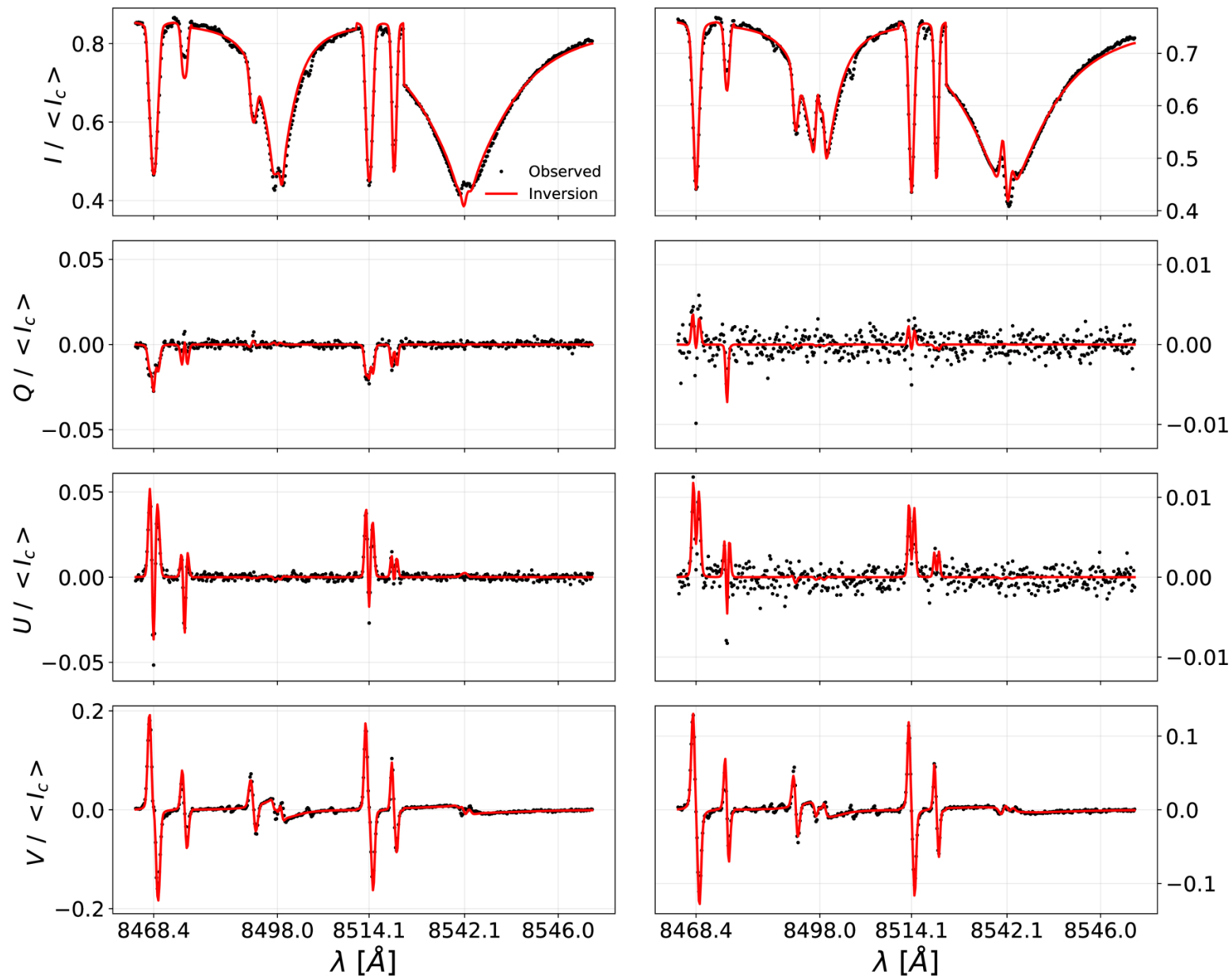
Figure 2. from Juan Carlos Trelles Arjona et al 2026 Astrophys. J. Lett. 1009 doi:10.3847/2041-8213/aea6c6 https://dx.doi.org/10.3847/2041-8213/aea6c6 © 2026. The Author(s). Published by the American Astronomical Society.
