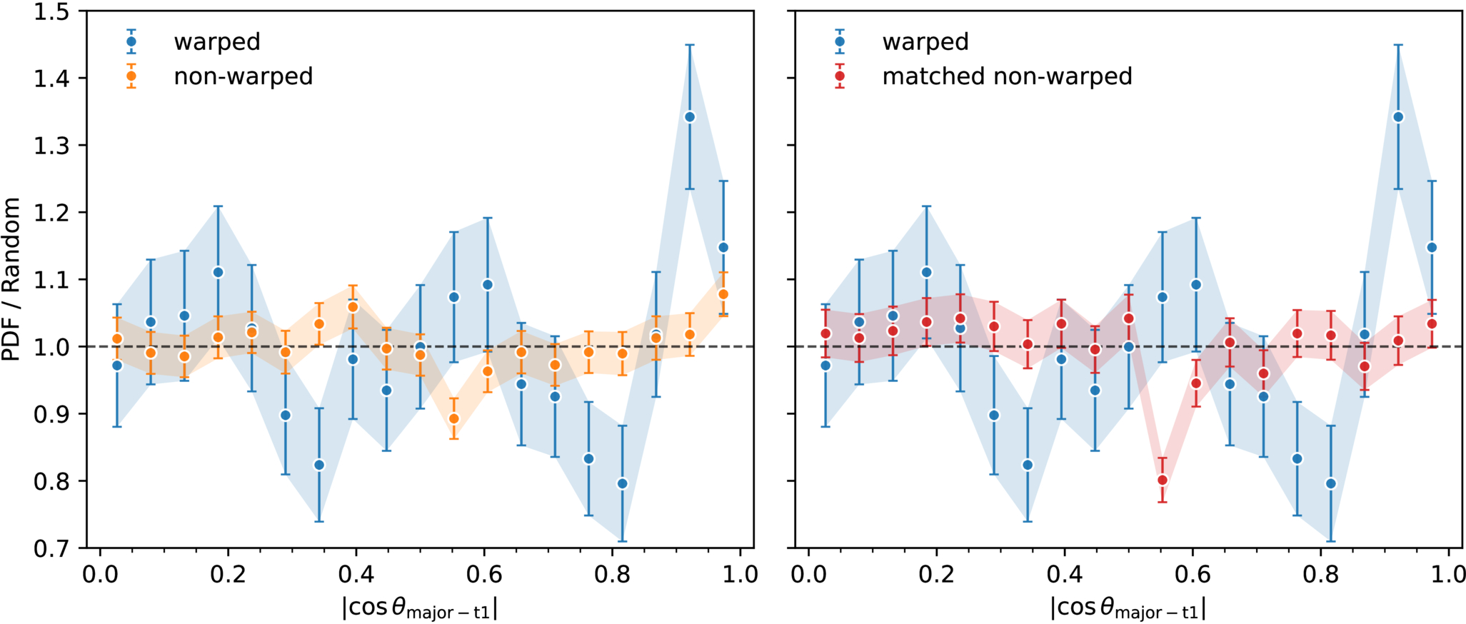
Figure 1. from Yiheng Wang et al 2026 Astrophys. J. Lett. 1009 doi:10.3847/2041-8213/aea6c2 https://dx.doi.org/10.3847/2041-8213/aea6c2 © 2026. The Author(s). Published by the American Astronomical Society.
