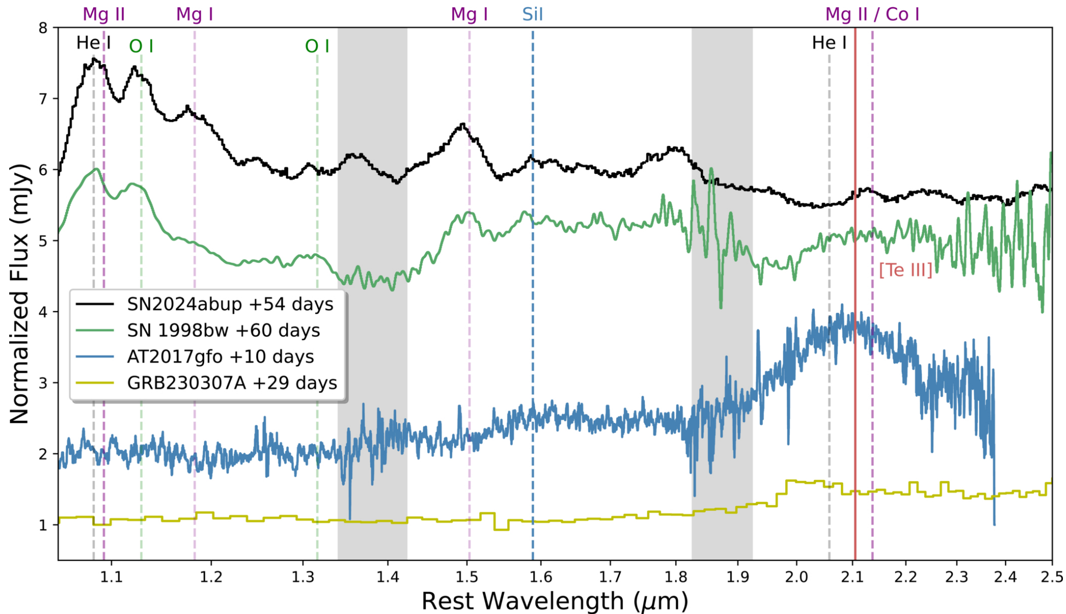
Figure 8. from Manisha Shrestha et al 2026 Astrophys. J. Lett. 1009 doi:10.3847/2041-8213/aea6bf https://dx.doi.org/10.3847/2041-8213/aea6bf © 2026. The Author(s). Published by the American Astronomical Society.
