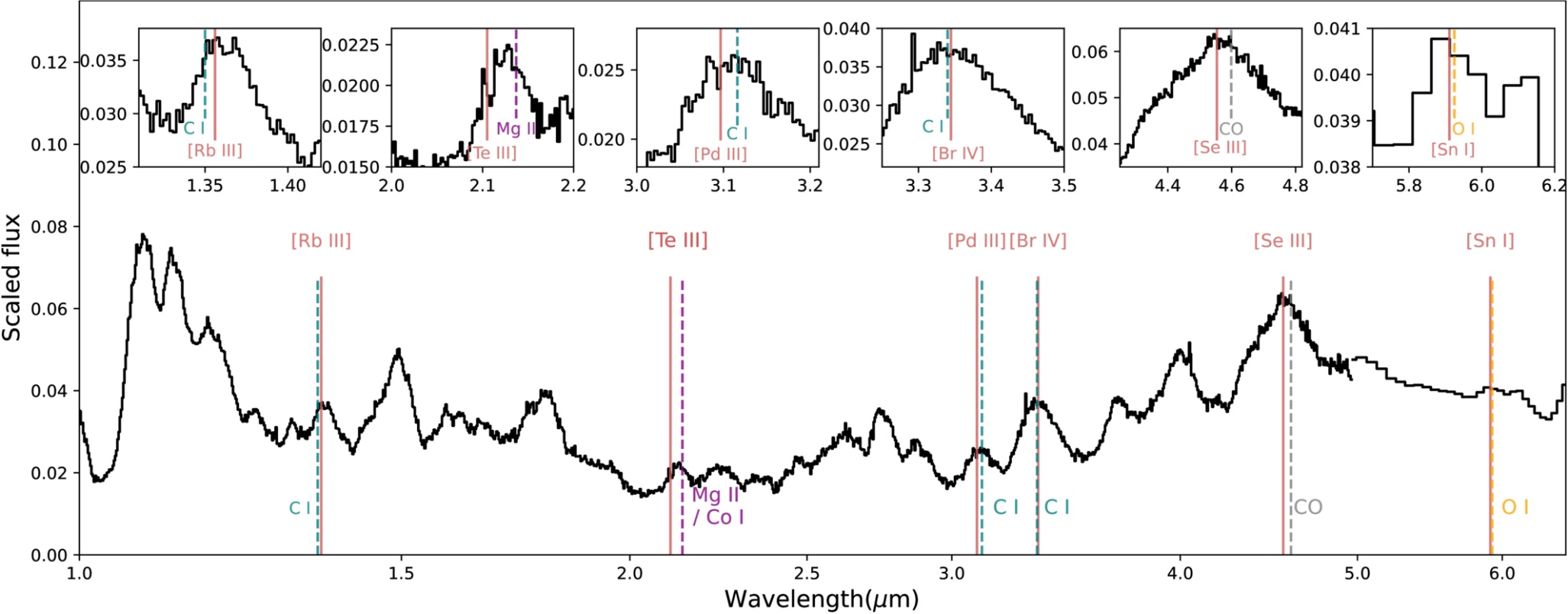
Figure 7. from Manisha Shrestha et al 2026 Astrophys. J. Lett. 1009 doi:10.3847/2041-8213/aea6bf https://dx.doi.org/10.3847/2041-8213/aea6bf © 2026. The Author(s). Published by the American Astronomical Society.
