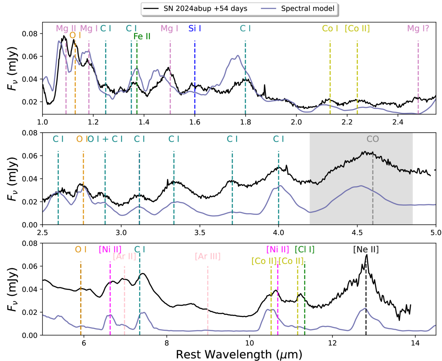
Figure 6. from Manisha Shrestha et al 2026 Astrophys. J. Lett. 1009 doi:10.3847/2041-8213/aea6bf https://dx.doi.org/10.3847/2041-8213/aea6bf © 2026. The Author(s). Published by the American Astronomical Society.
