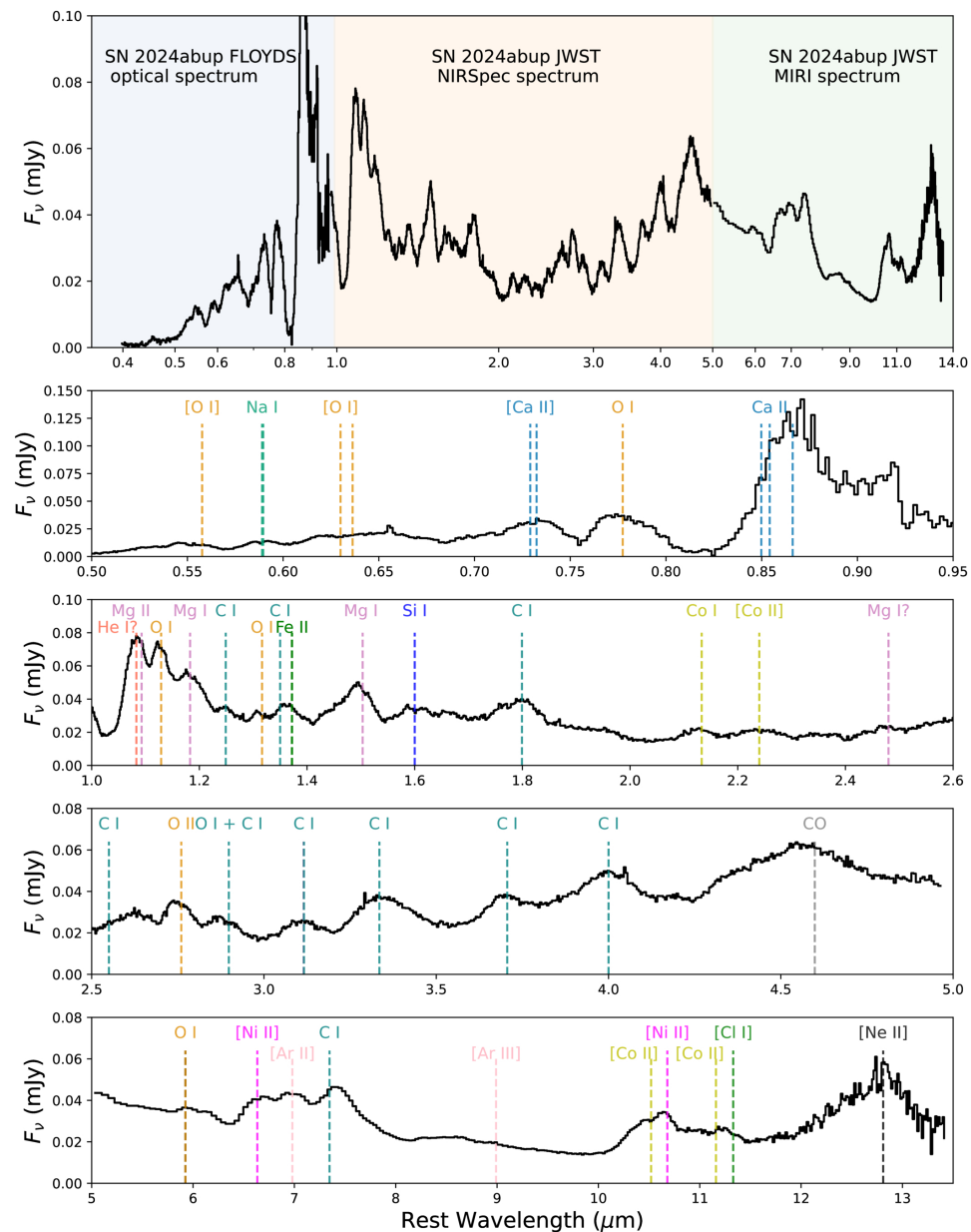
Figure 3. from Manisha Shrestha et al 2026 Astrophys. J. Lett. 1009 doi:10.3847/2041-8213/aea6bf https://dx.doi.org/10.3847/2041-8213/aea6bf © 2026. The Author(s). Published by the American Astronomical Society.
