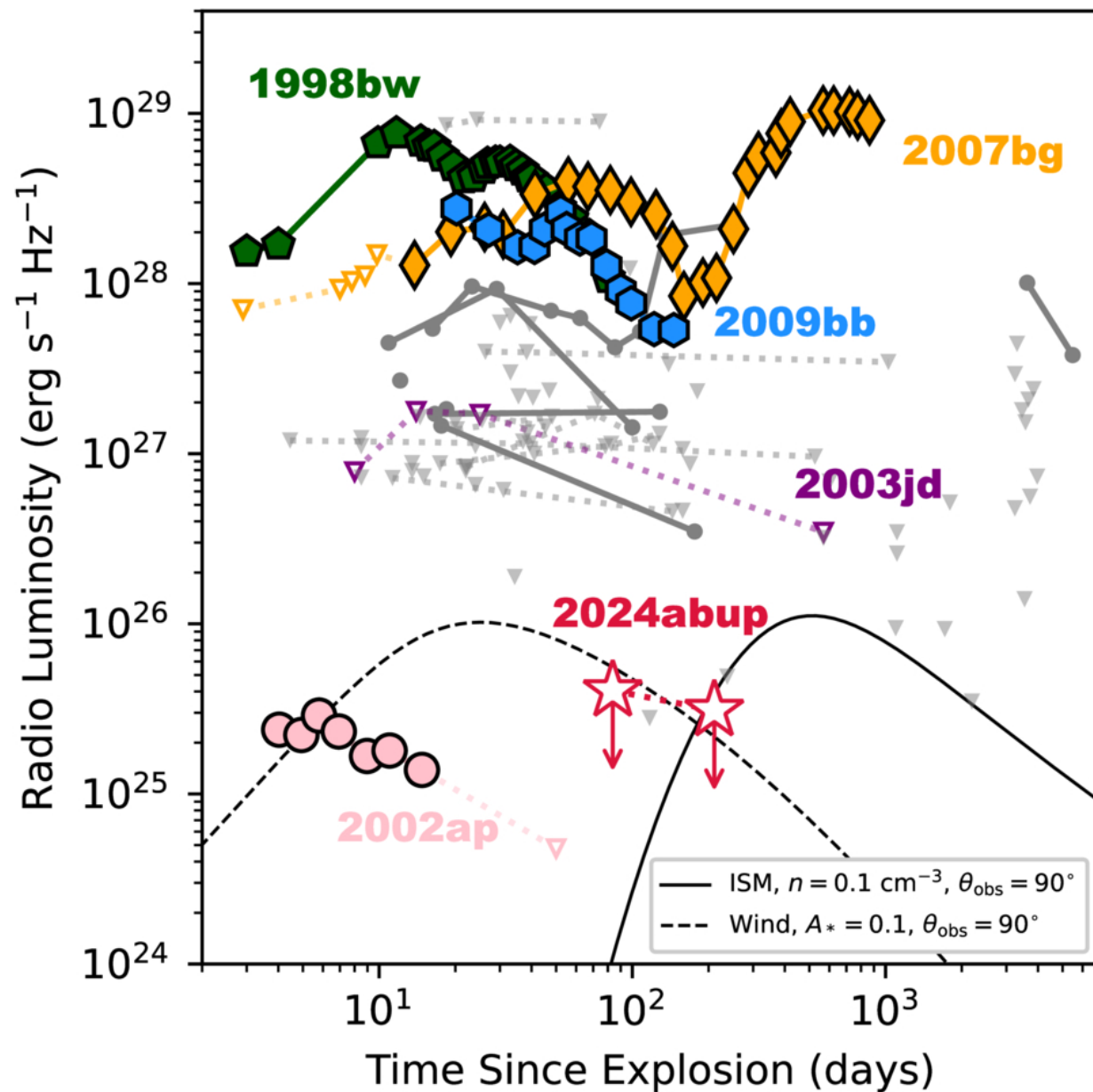
Figure 11. from Manisha Shrestha et al 2026 Astrophys. J. Lett. 1009 doi:10.3847/2041-8213/aea6bf https://dx.doi.org/10.3847/2041-8213/aea6bf © 2026. The Author(s). Published by the American Astronomical Society.
