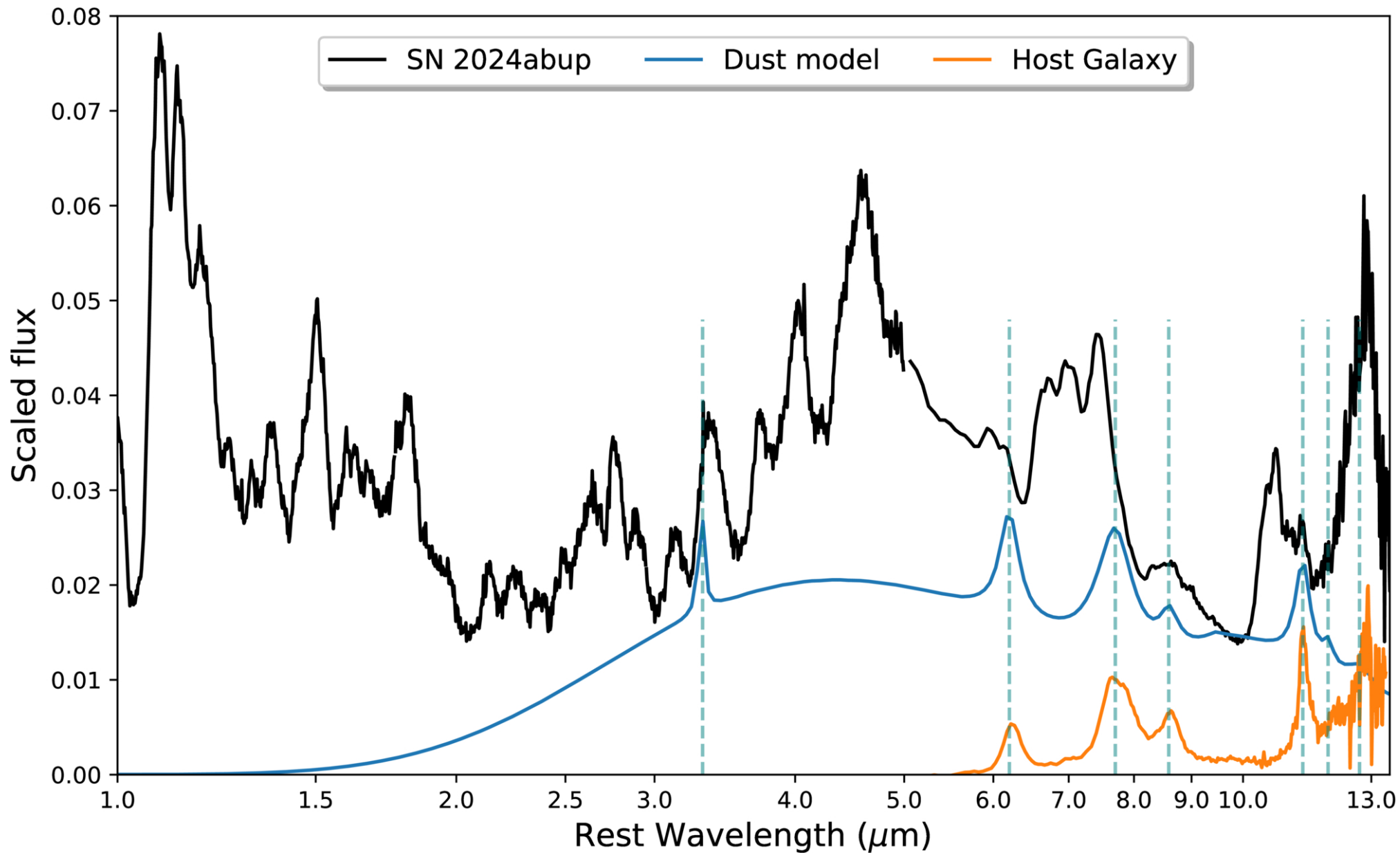
Figure 10. from Manisha Shrestha et al 2026 Astrophys. J. Lett. 1009 doi:10.3847/2041-8213/aea6bf https://dx.doi.org/10.3847/2041-8213/aea6bf © 2026. The Author(s). Published by the American Astronomical Society.
