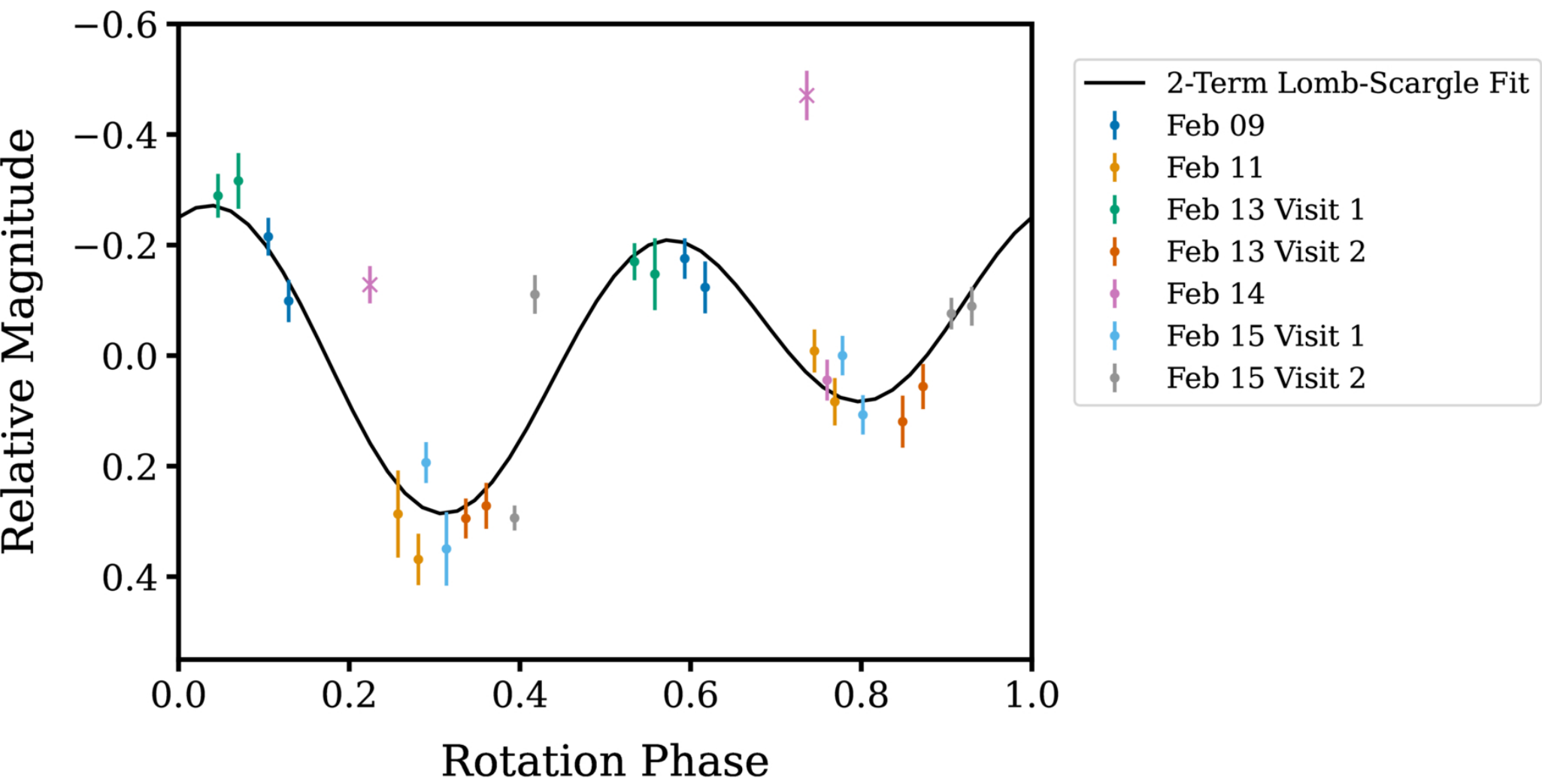
Figure 2. from Benjamin N. L. Sharkey et al 2026 Astrophys. J. Lett. 1010 doi:10.3847/2041-8213/aea6b6 https://dx.doi.org/10.3847/2041-8213/aea6b6 © 2026. The Author(s). Published by the American Astronomical Society.
