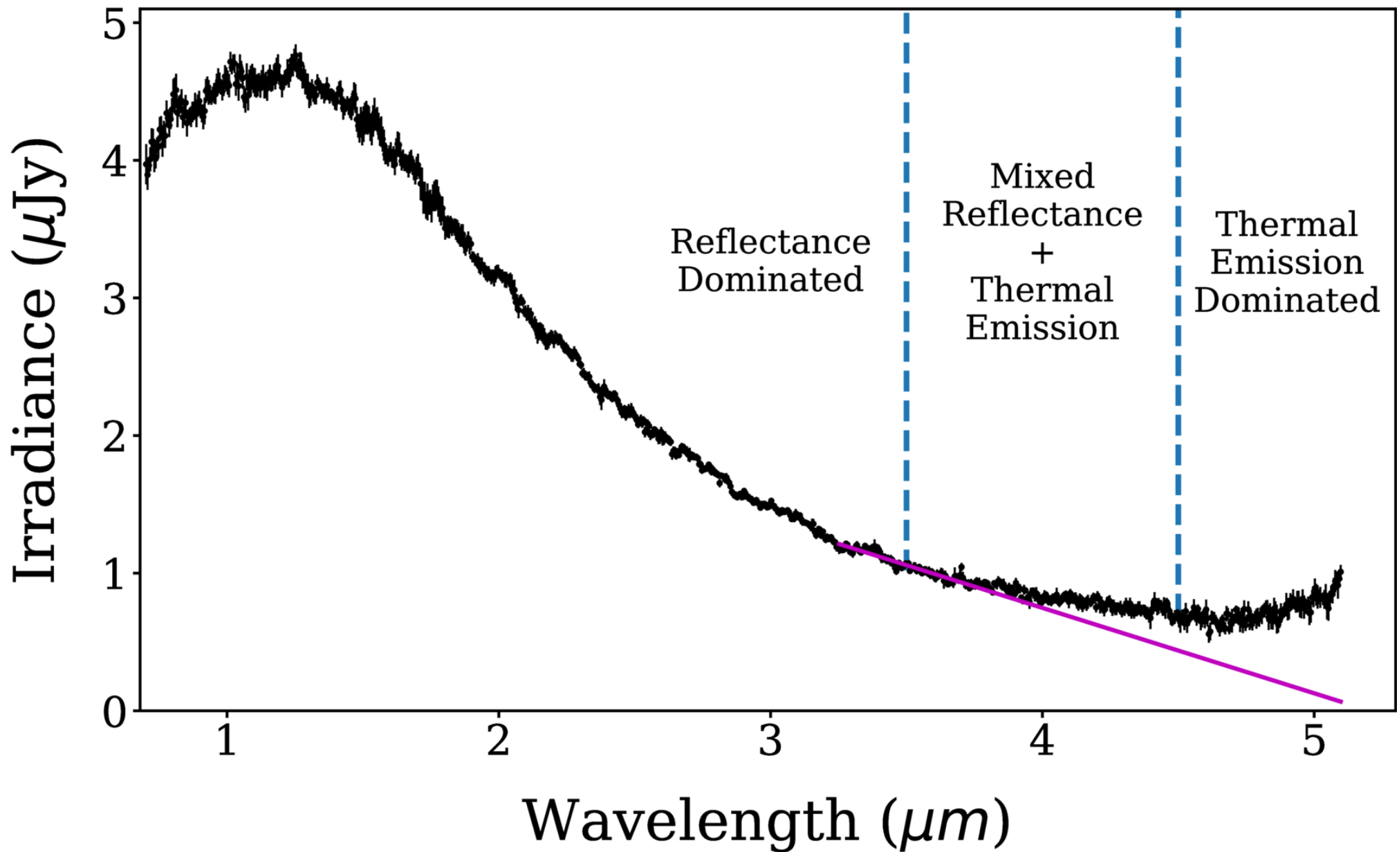
Figure 1. from Benjamin N. L. Sharkey et al 2026 Astrophys. J. Lett. 1010 doi:10.3847/2041-8213/aea6b6 https://dx.doi.org/10.3847/2041-8213/aea6b6 © 2026. The Author(s). Published by the American Astronomical Society.
