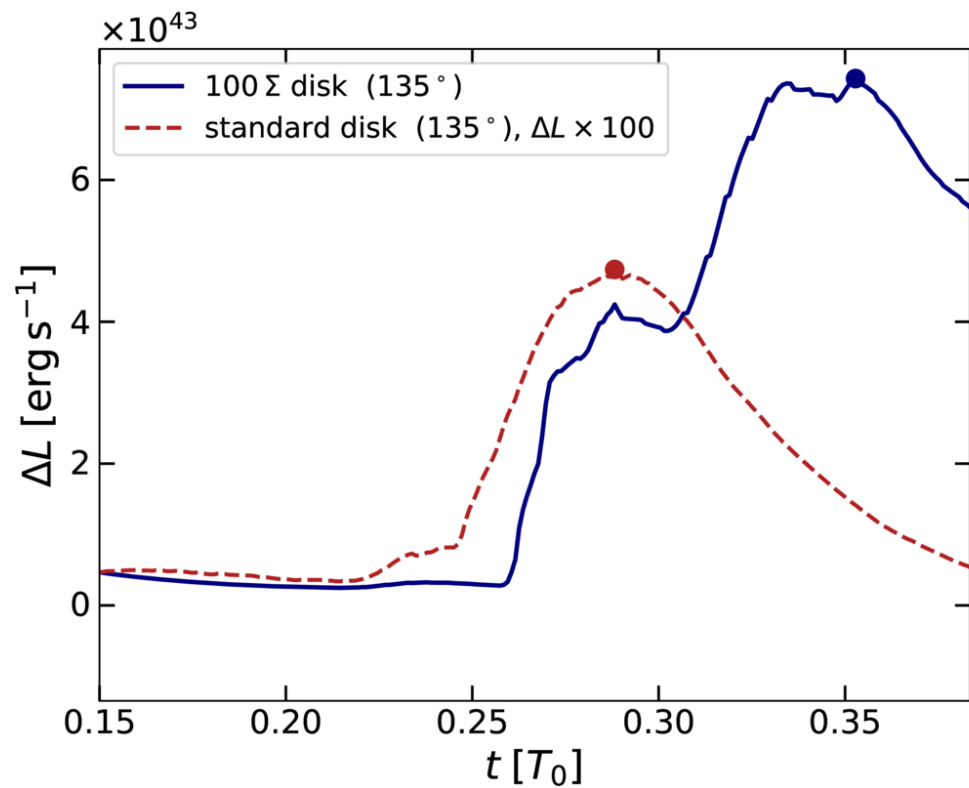
Figure 6. from Zhaohuan Zhu et al 2026 Astrophys. J. Lett. 1009 doi:10.3847/2041-8213/aea6a1 https://dx.doi.org/10.3847/2041-8213/aea6a1 © 2026. The Author(s). Published by the American Astronomical Society.
