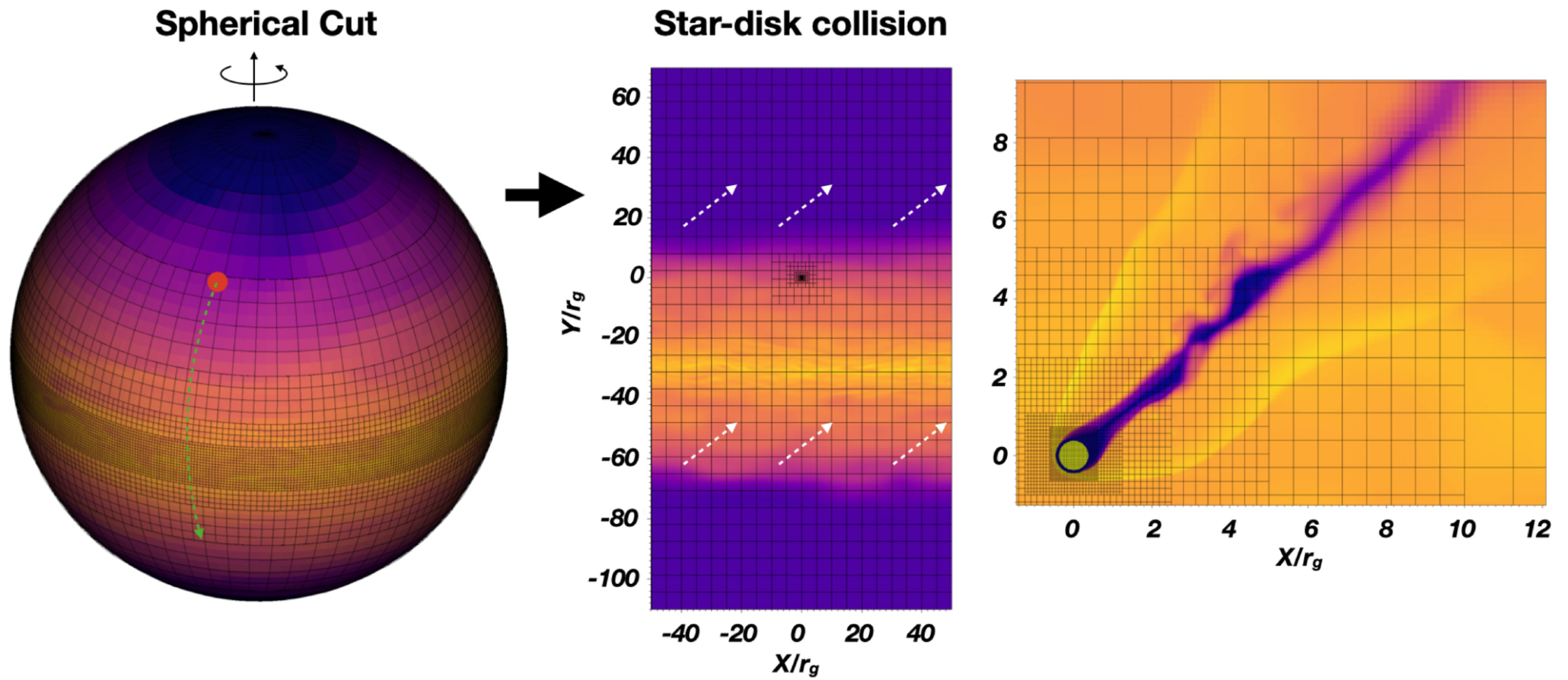
Figure 1. from Zhaohuan Zhu et al 2026 Astrophys. J. Lett. 1009 doi:10.3847/2041-8213/aea6a1 https://dx.doi.org/10.3847/2041-8213/aea6a1 © 2026. The Author(s). Published by the American Astronomical Society.
