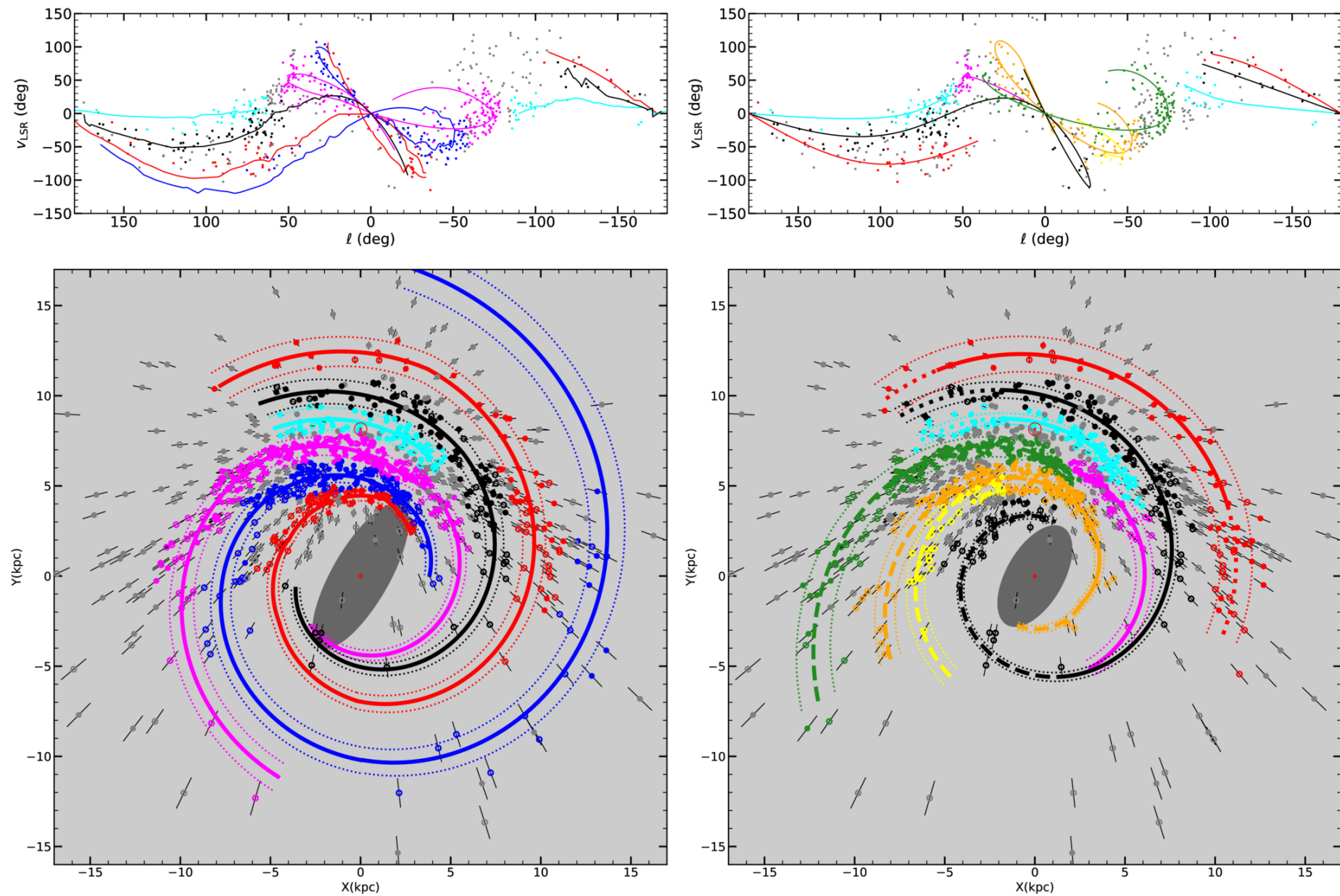
Figure 2. from Z. H. Lin et al 2026 Astrophys. J. Lett. 1009 doi:10.3847/2041-8213/aea61c https://dx.doi.org/10.3847/2041-8213/aea61c © 2026. The Author(s). Published by the American Astronomical Society.
