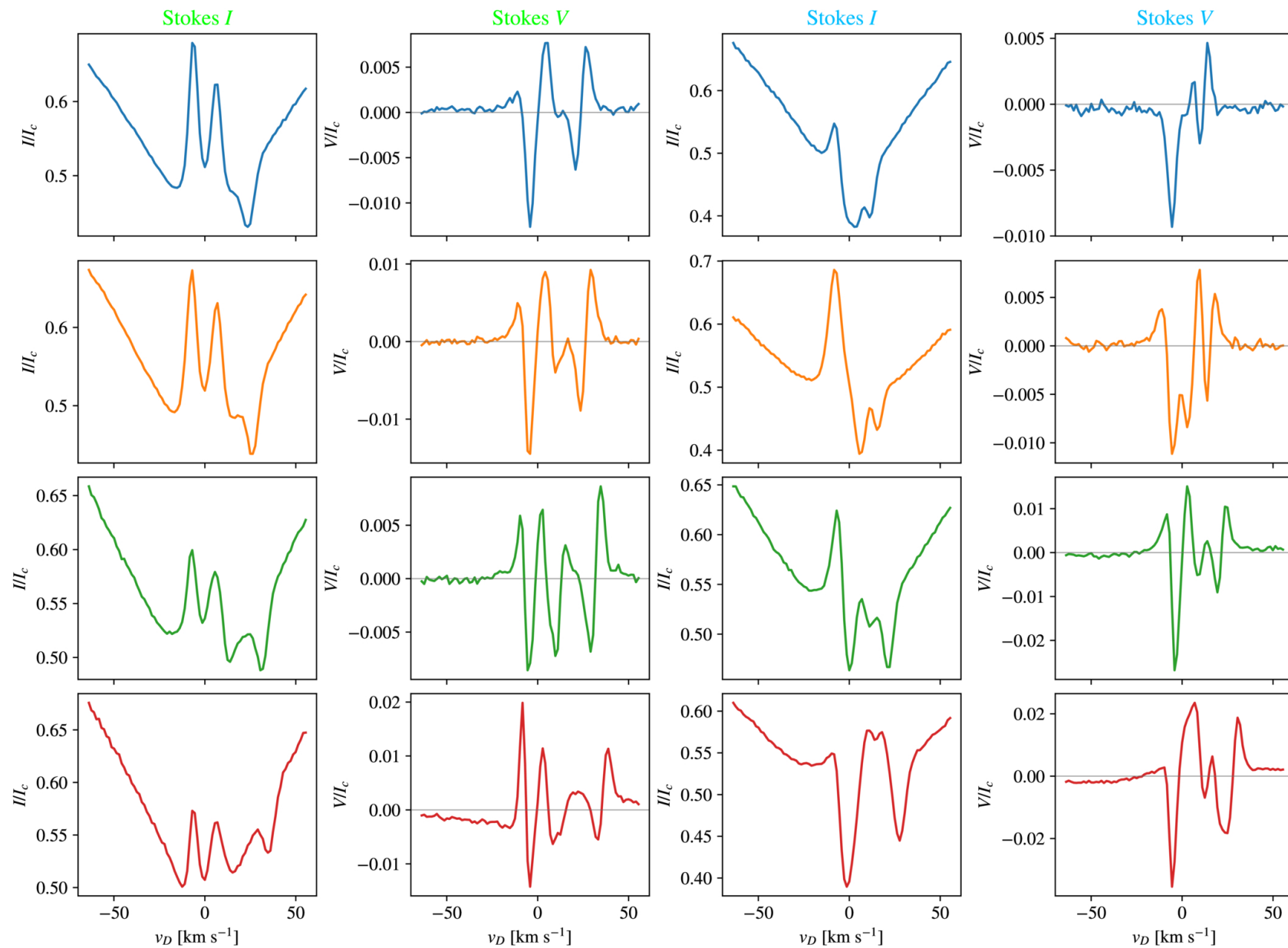
Figure A1. from Matheus Kriginsky et al 2026 Astrophys. J. Lett. 1009 doi:10.3847/2041-8213/aea575 https://dx.doi.org/10.3847/2041-8213/aea575 © 2026. The Author(s). Published by the American Astronomical Society.
