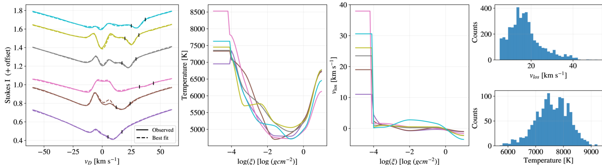
Figure 3. from Matheus Kriginsky et al 2026 Astrophys. J. Lett. 1009 doi:10.3847/2041-8213/aea575 https://dx.doi.org/10.3847/2041-8213/aea575 © 2026. The Author(s). Published by the American Astronomical Society.
