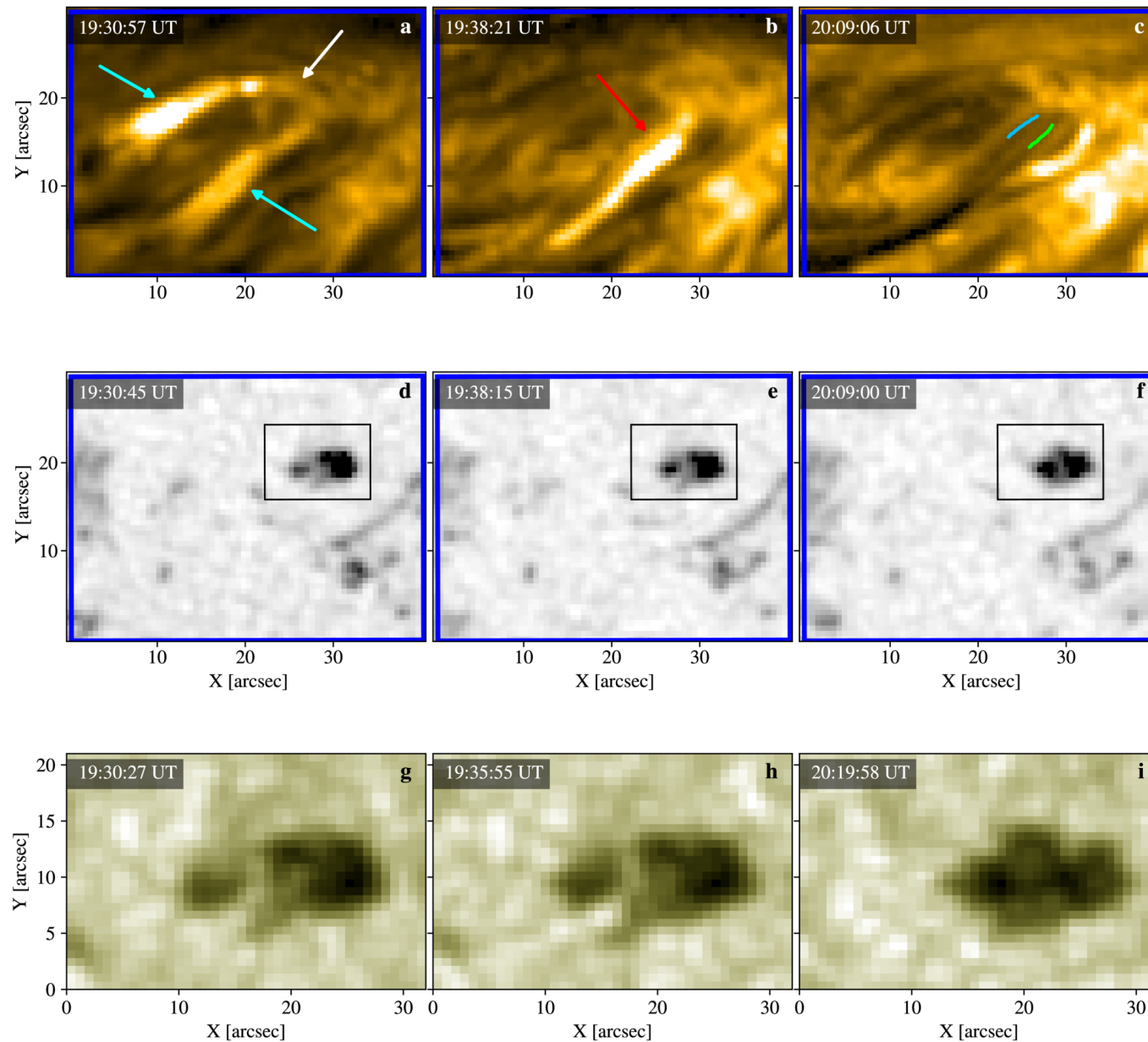
Figure 2. from Matheus Kriginsky et al 2026 Astrophys. J. Lett. 1009 doi:10.3847/2041-8213/aea575 https://dx.doi.org/10.3847/2041-8213/aea575 © 2026. The Author(s). Published by the American Astronomical Society.
