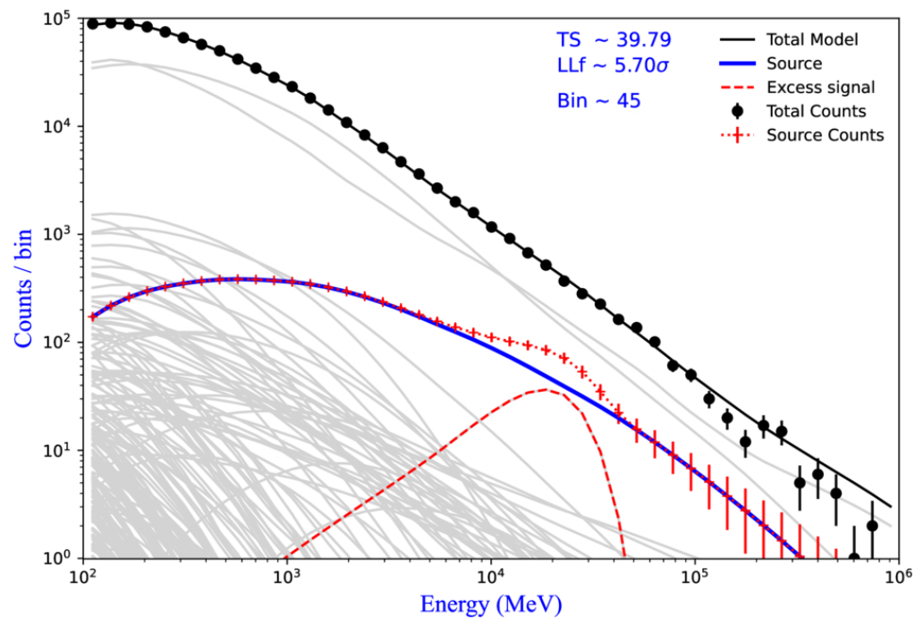
Figure 2. from Shi-Ju Kang et al 2026 Astrophys. J. Lett. 1009 doi:10.3847/2041-8213/aea572 https://dx.doi.org/10.3847/2041-8213/aea572 © 2026. The Author(s). Published by the American Astronomical Society.
