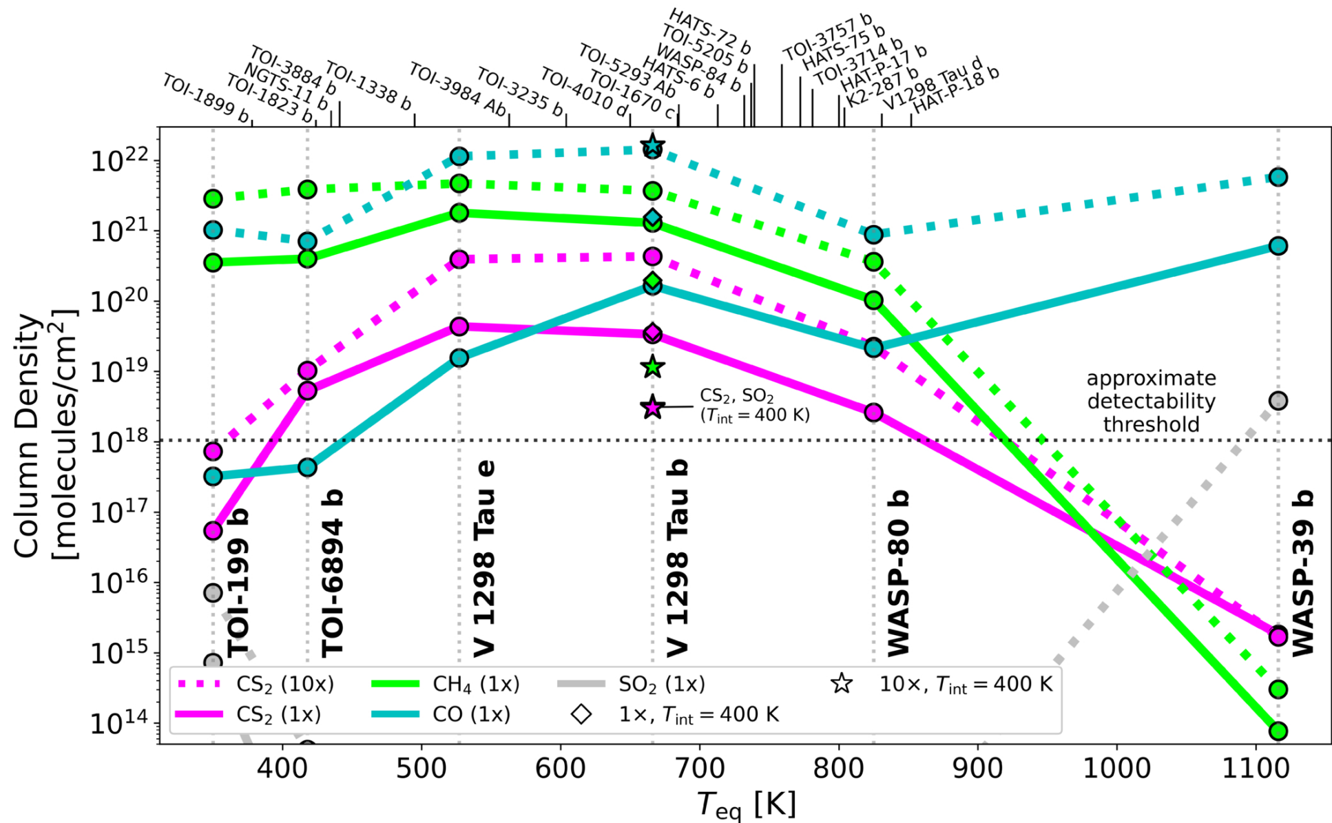
Figure 5. from Jeehyun Yang et al 2026 Astrophys. J. Lett. 1009 doi:10.3847/2041-8213/aea4af https://dx.doi.org/10.3847/2041-8213/aea4af © 2026. The Author(s). Published by the American Astronomical Society.
