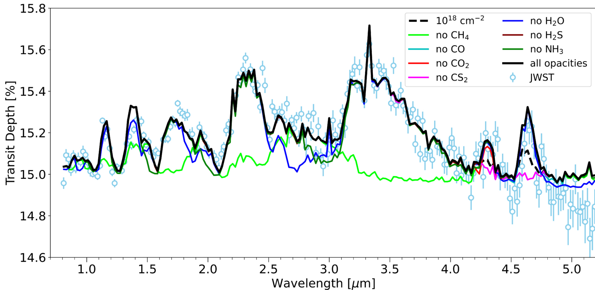
Figure 4. from Jeehyun Yang et al 2026 Astrophys. J. Lett. 1009 doi:10.3847/2041-8213/aea4af https://dx.doi.org/10.3847/2041-8213/aea4af © 2026. The Author(s). Published by the American Astronomical Society.
