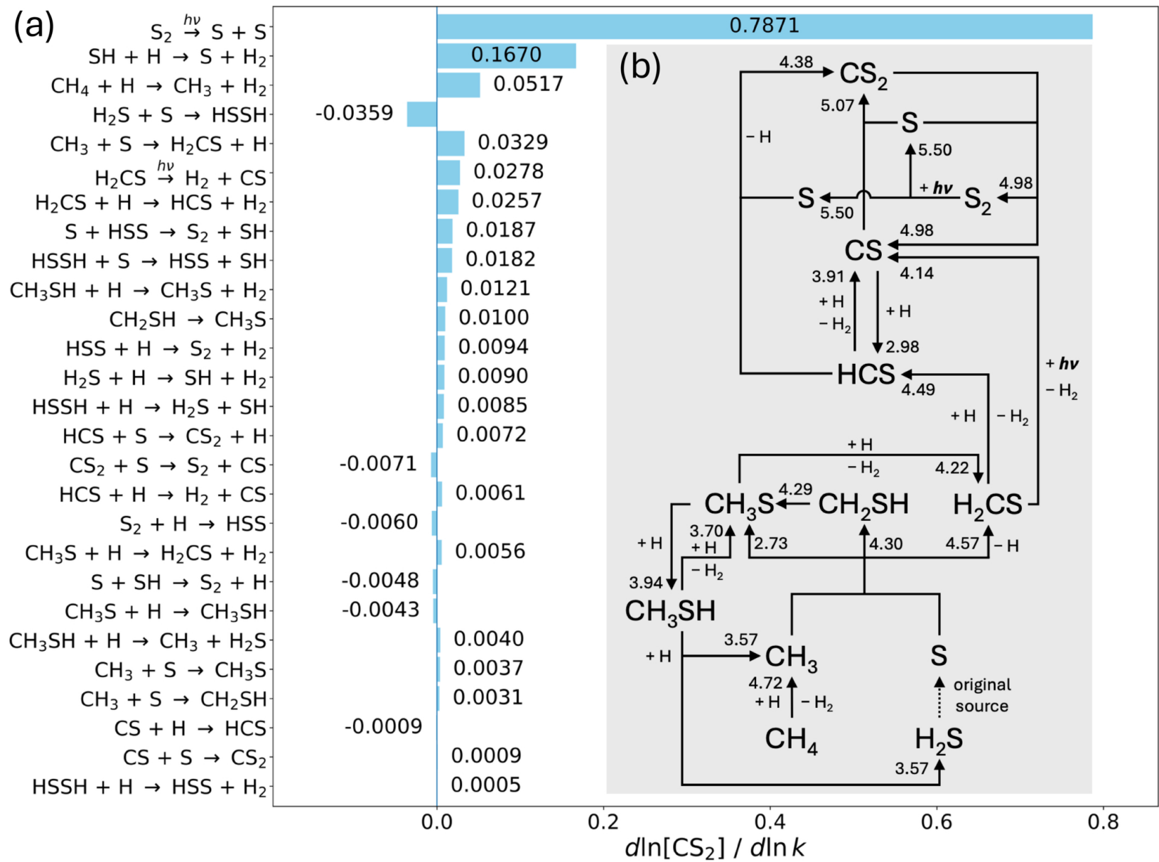
Figure 2. from Jeehyun Yang et al 2026 Astrophys. J. Lett. 1009 doi:10.3847/2041-8213/aea4af https://dx.doi.org/10.3847/2041-8213/aea4af © 2026. The Author(s). Published by the American Astronomical Society.
