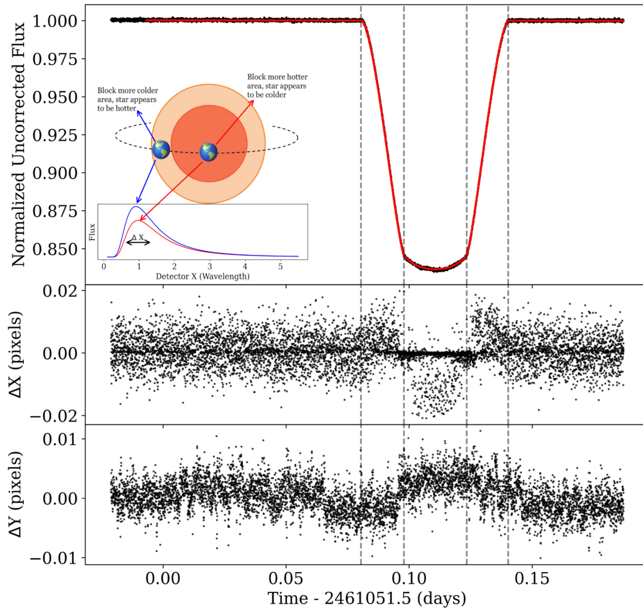
Figure A1. from Michael Zhang et al 2026 Astrophys. J. Lett. 1009 doi:10.3847/2041-8213/aea4ae https://dx.doi.org/10.3847/2041-8213/aea4ae © 2026. The Author(s). Published by the American Astronomical Society.
