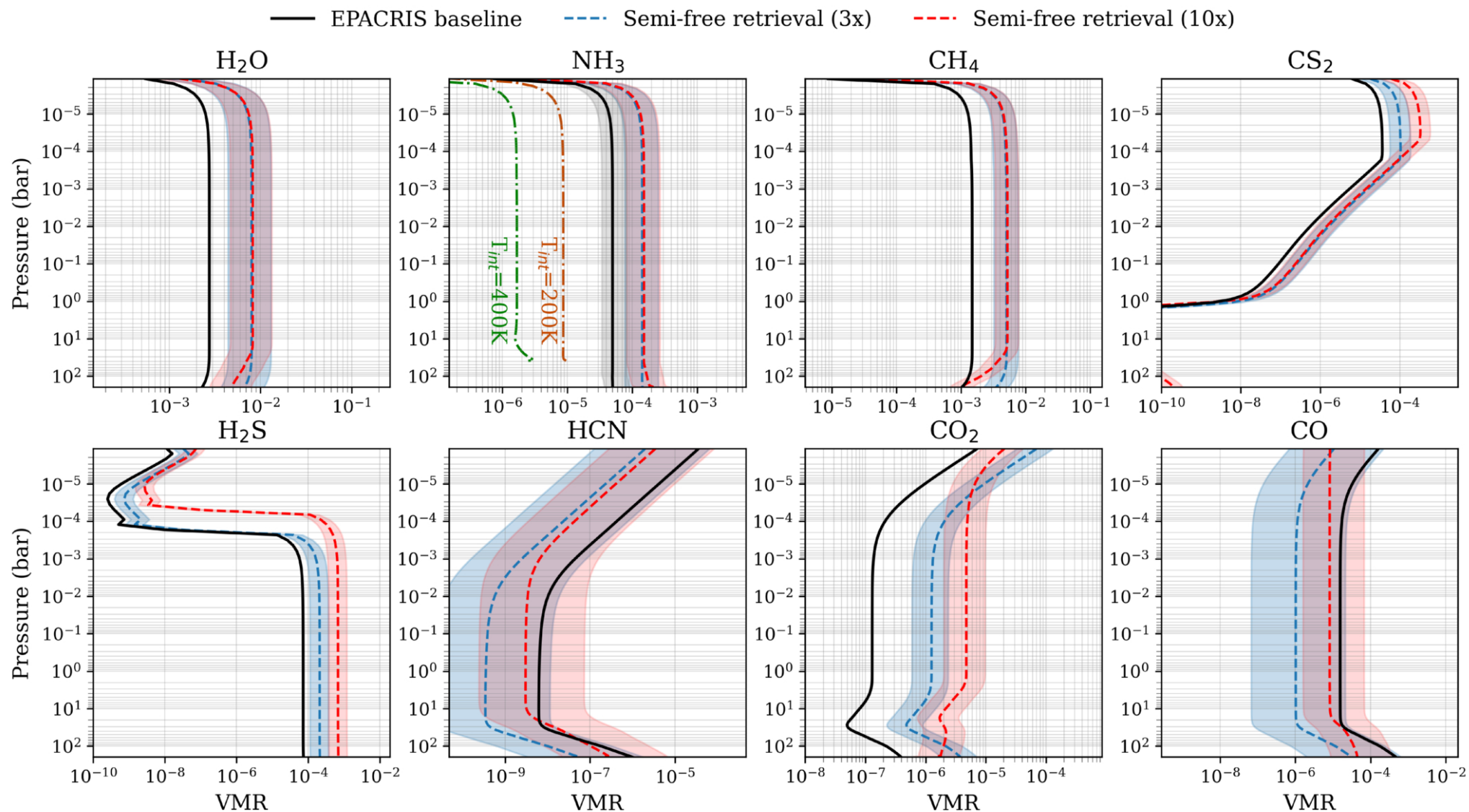
Figure 3. from Michael Zhang et al 2026 Astrophys. J. Lett. 1009 doi:10.3847/2041-8213/aea4ae https://dx.doi.org/10.3847/2041-8213/aea4ae © 2026. The Author(s). Published by the American Astronomical Society.
