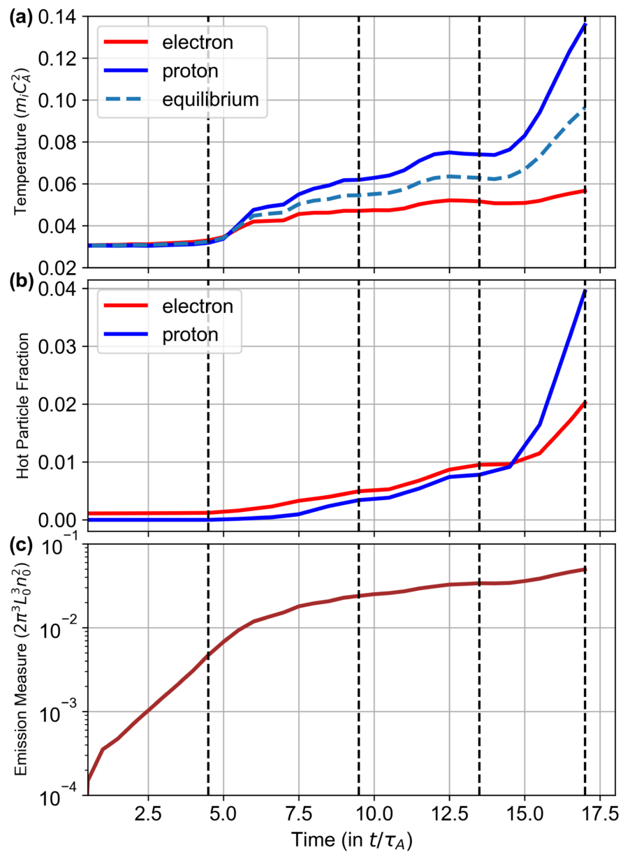
Figure 4. from H. Da et al 2026 Astrophys. J. Lett. 1009 doi:10.3847/2041-8213/aea4ad https://dx.doi.org/10.3847/2041-8213/aea4ad © 2026. The Author(s). Published by the American Astronomical Society.
