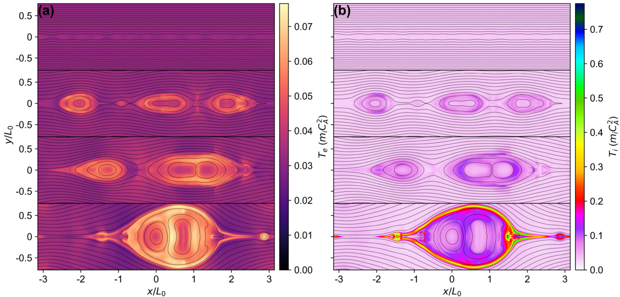
Figure 2. from H. Da et al 2026 Astrophys. J. Lett. 1009 doi:10.3847/2041-8213/aea4ad https://dx.doi.org/10.3847/2041-8213/aea4ad © 2026. The Author(s). Published by the American Astronomical Society.
