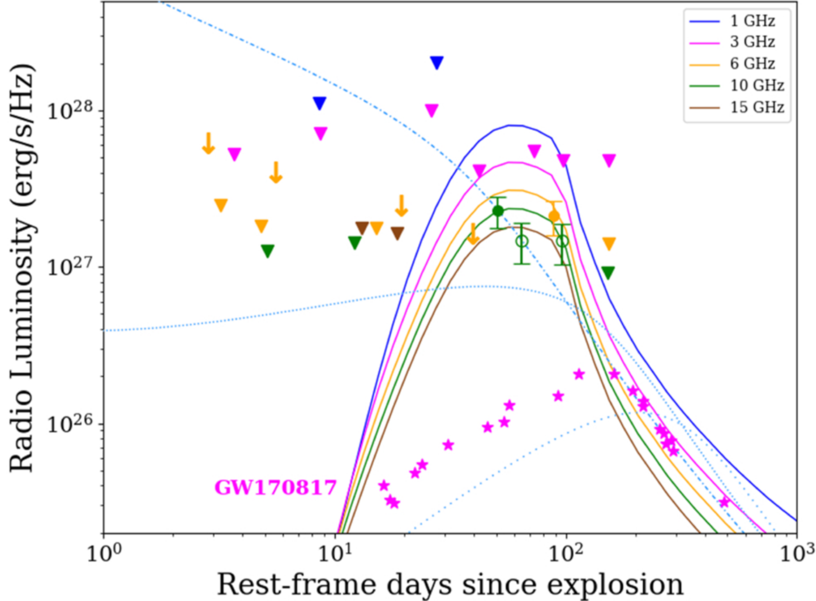
Figure 4. from Tanner O'Dwyer et al 2026 Astrophys. J. Lett. 1009 doi:10.3847/2041-8213/aea4a5 https://dx.doi.org/10.3847/2041-8213/aea4a5 © 2026. The Author(s). Published by the American Astronomical Society.
