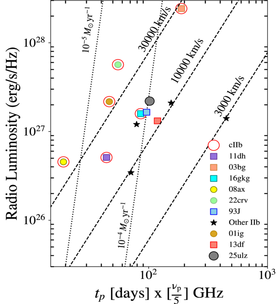
Figure 3. from Tanner O'Dwyer et al 2026 Astrophys. J. Lett. 1009 doi:10.3847/2041-8213/aea4a5 https://dx.doi.org/10.3847/2041-8213/aea4a5 © 2026. The Author(s). Published by the American Astronomical Society.
