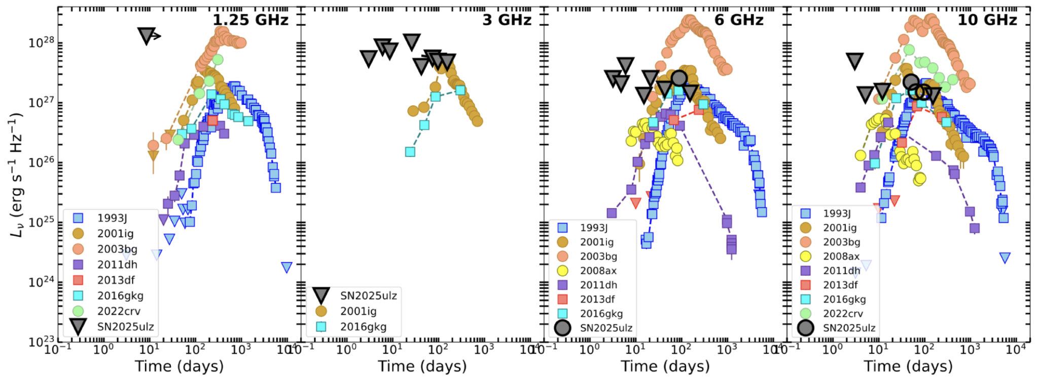
Figure 2. from Tanner O'Dwyer et al 2026 Astrophys. J. Lett. 1009 doi:10.3847/2041-8213/aea4a5 https://dx.doi.org/10.3847/2041-8213/aea4a5 © 2026. The Author(s). Published by the American Astronomical Society.
