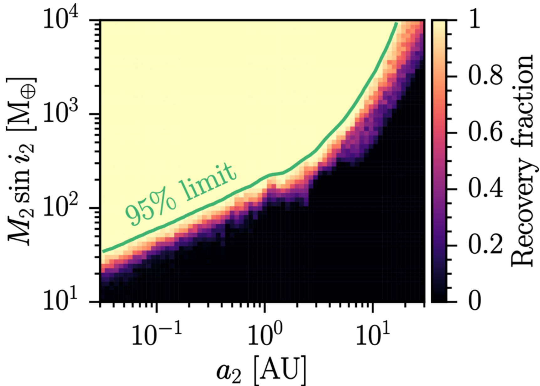
Figure 3. from Caleb Lammers et al 2026 Astrophys. J. Lett. 1009 doi:10.3847/2041-8213/aea405 https://dx.doi.org/10.3847/2041-8213/aea405 © 2026. The Author(s). Published by the American Astronomical Society.
