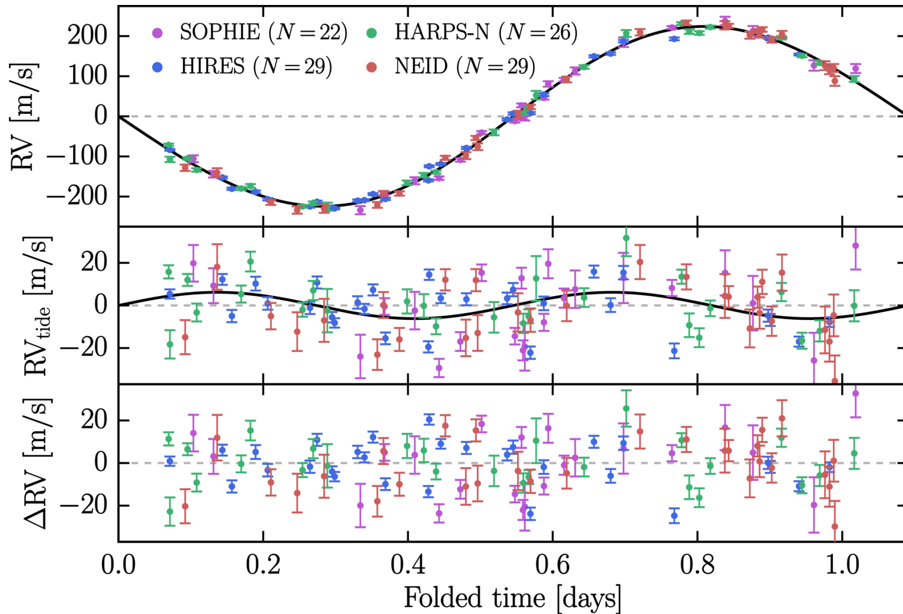
Figure 2. from Caleb Lammers et al 2026 Astrophys. J. Lett. 1009 doi:10.3847/2041-8213/aea405 https://dx.doi.org/10.3847/2041-8213/aea405 © 2026. The Author(s). Published by the American Astronomical Society.
