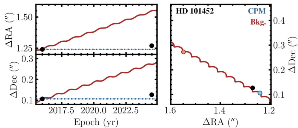
(a) Common proper motion verification
