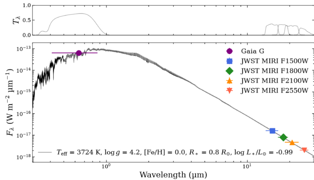
(b) Spectral energy distribution fit
