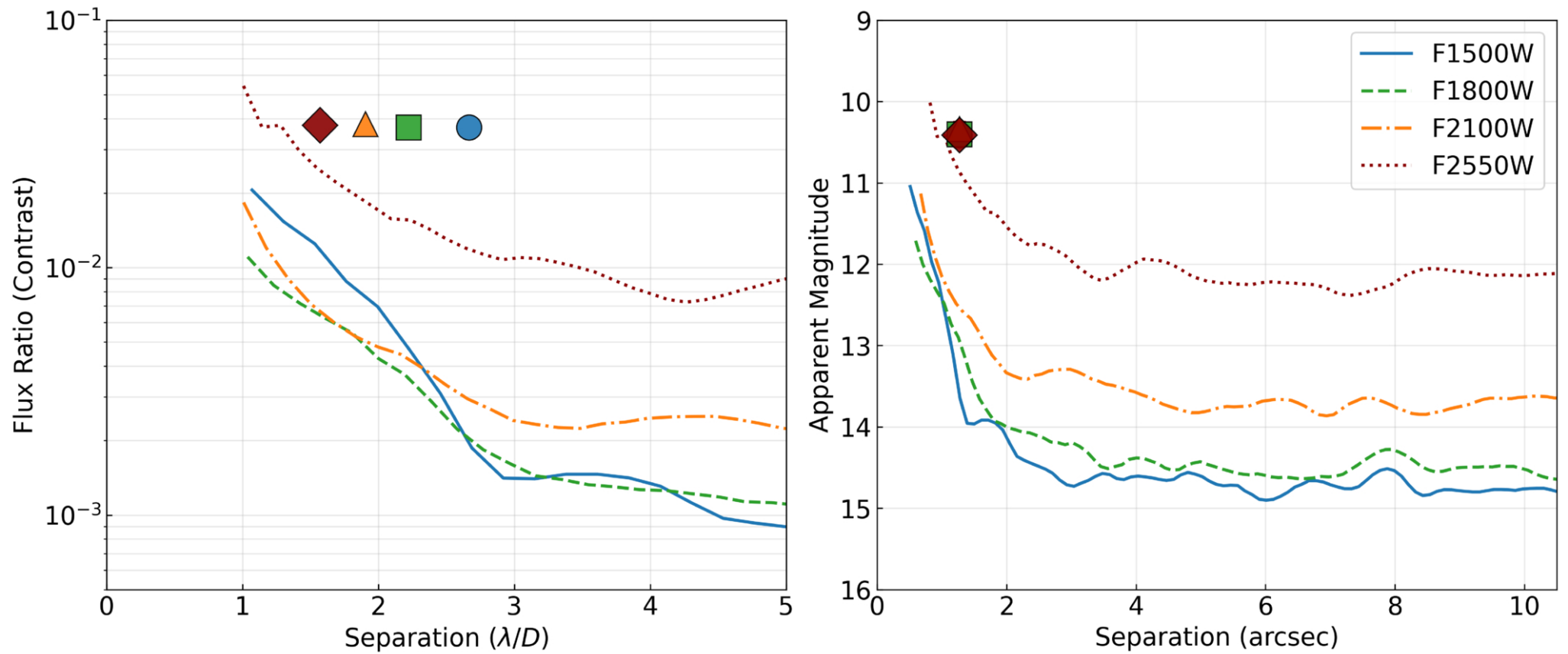
Figure 2. from Rachel Bowens-Rubin et al 2026 Astrophys. J. Lett. 1009 doi:10.3847/2041-8213/aea3f5 https://dx.doi.org/10.3847/2041-8213/aea3f5 © 2026. The Author(s). Published by the American Astronomical Society.
